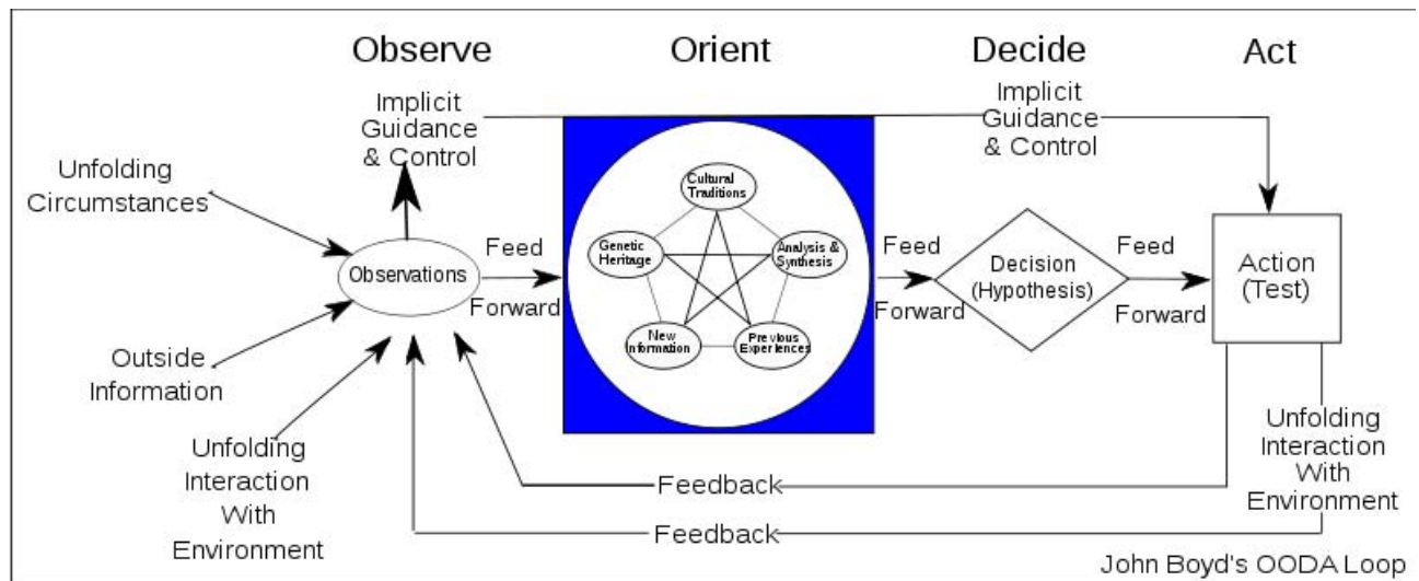
Figure 4. OODA-Loop
