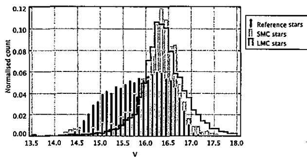
Figure 9. Histogram of V magnitude for the reference stars, LMC and SMC stars. All three data sets overlap substantially in V , which helps to reduce systematics in the proper motions related to brightness.
