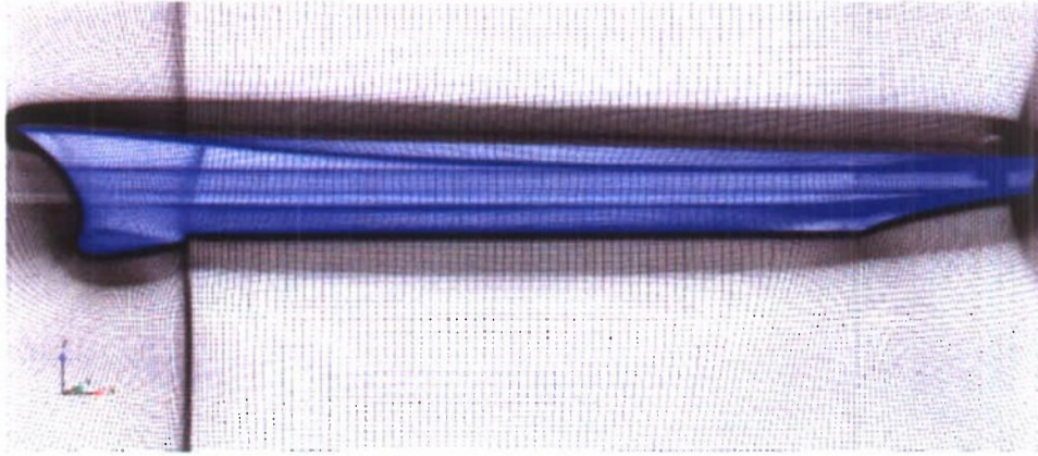
Figure 41. Grid for DTMB Model 5415
