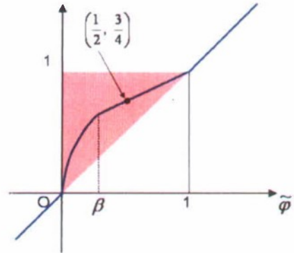
Figure 8. NVD of Gamma scheme with CBC
