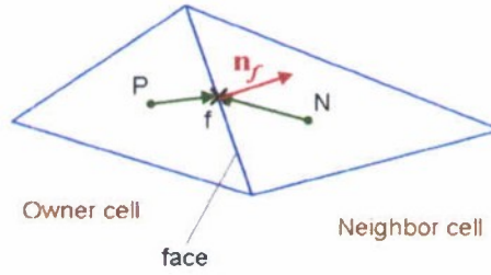
Figure 20. Calculating face-normal gradient
