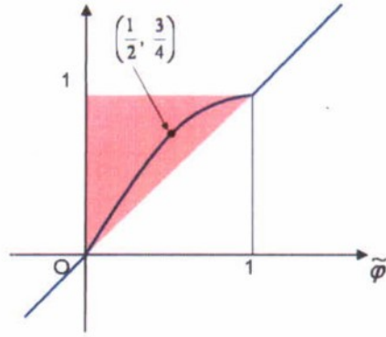
Figure 7. NVD of vanLeer scheme with CBC
