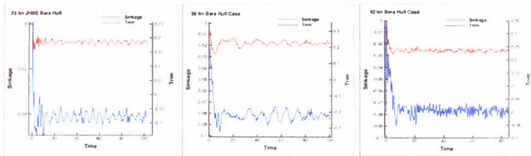
Figure 51. Sinkage and trim run time values plotted for three different Froude numbers
