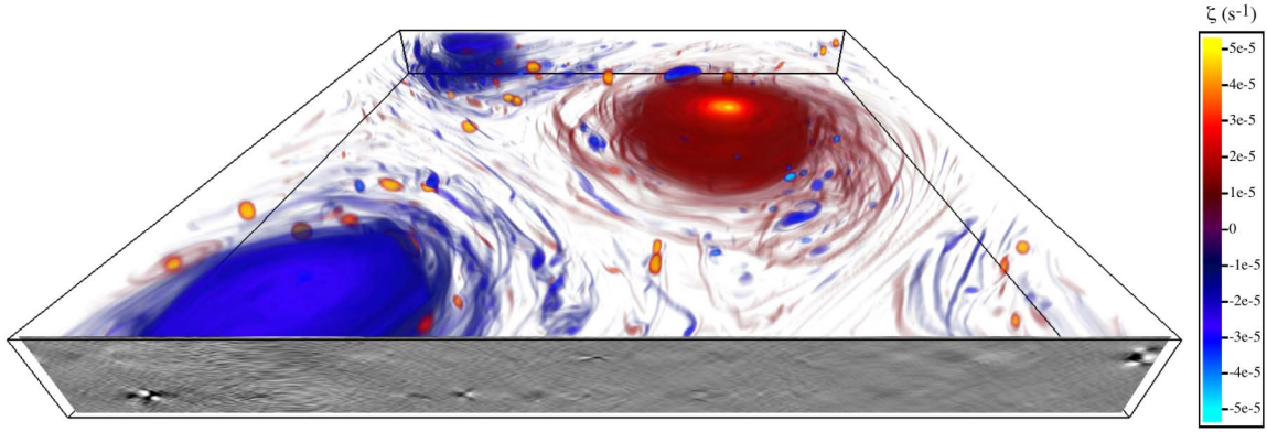
Figure 4: Vertical vorticity (color shading) from the NHB model at t=146 days. At this time the large scales have coalesced into a dipole consisting of a strong cyclone, and a somewhat weaker anticyclone. Despite the inverse energy cascade, small-scale filaments and eddies are clearly visible. The front plane shows the vertical divergence field, dw/dz , which highlights the internal wave field and sub-mesoscale features.
