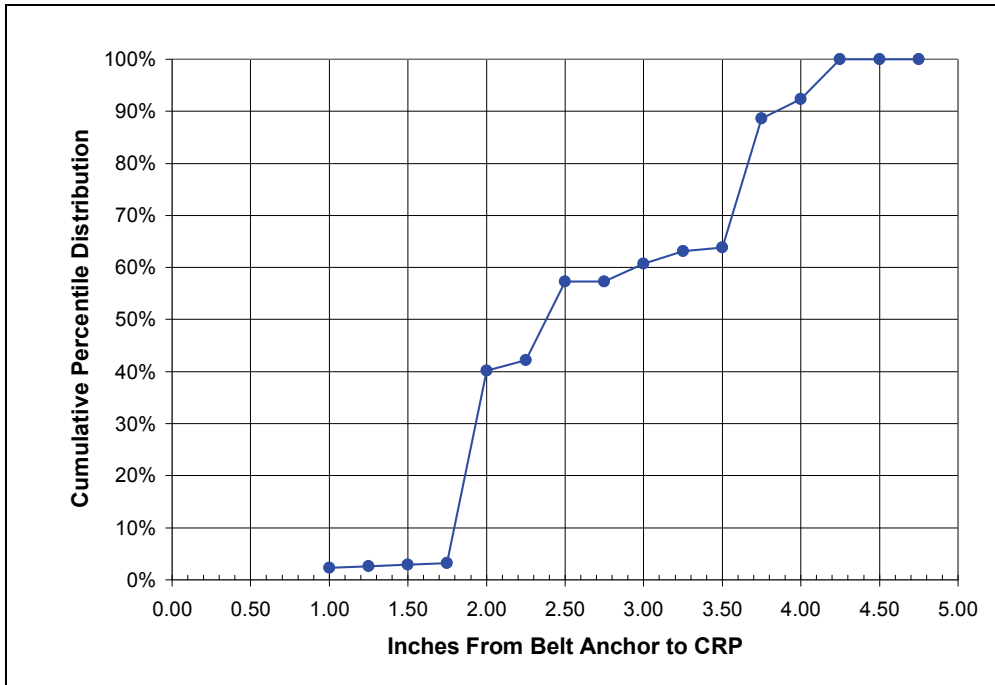
Figure 4 – CRP-to-Lap Belt Anchor Horizontal Distance, Cumulative Percentile Distribution - Current Conservative Estimate
