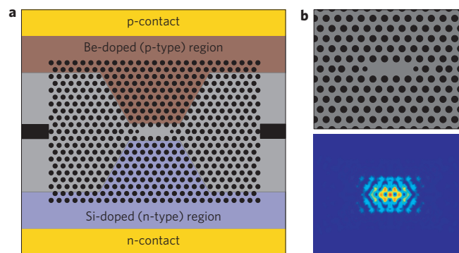
Figure 1 | Design of the electrically pumped photonic-crystal laser.
