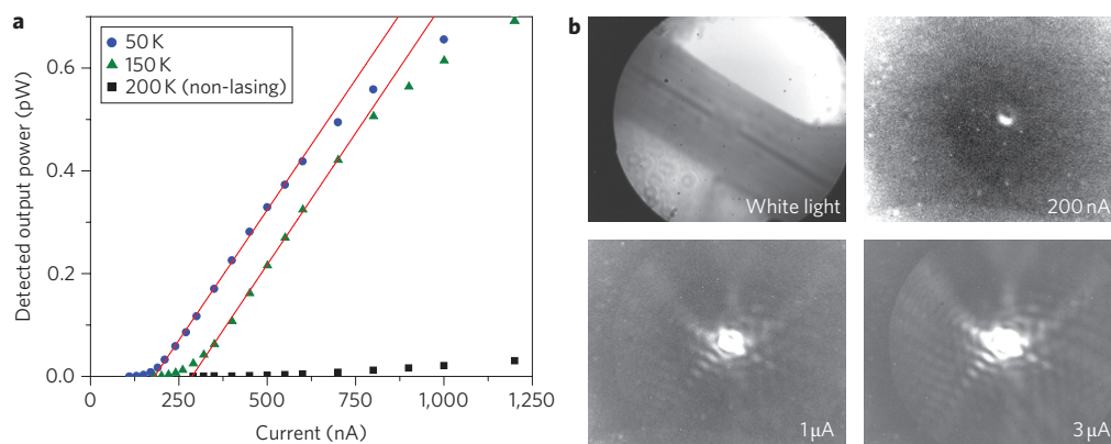
Figure 3 | Optical output of the photonic-crystal laser. a , Experimental output power (detected on the spectrometer) as a function of the current through the laser at 50 K (blue points), 150 K (green points) and 200 K (non-lasing; black points). Red lines are linear fits to the above threshold output power of the lasers, which are used to find the thresholds. We estimate from the collected output power that the total radiated power of the laser above threshold is on the order of a few nanowatts. b , Far-field radiation patterns of the laser at currents of 200 nA, 1 \mu A and 3 \mu A taken at 50 K. A white light image of the cavity is also shown. The n-contact is in the lower left corner of the image, and the p-contact in the upper right.
