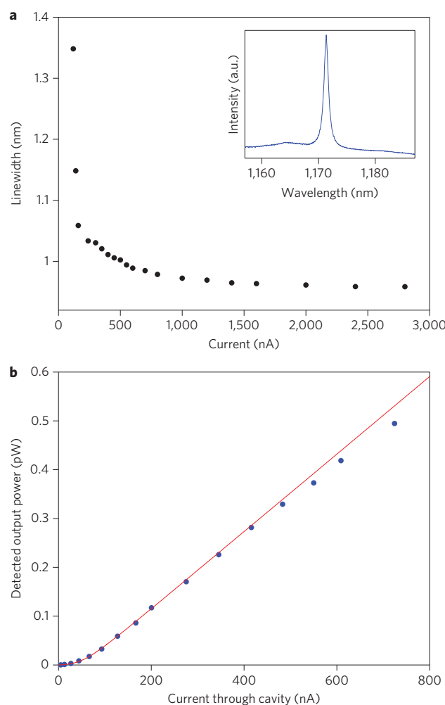
Figure 4 | Optical properties of the photonic-crystal laser. a , Linewidth of the photonic-crystal laser as a function of current. Inset: spectrum of the photonic-crystal laser at a pump current of 1 \mu A. b , This figure re-plots the data shown in Fig. 3a for 50 K after subtracting the leakage current of the diode (blue points); the result is then fitted to the laser rate equations (red line). ‘Current through cavity’ (on the horizontal axis) refers to the current flowing through the cavity region after subtracting leakage through the substrate (see text and Supplementary Information).
