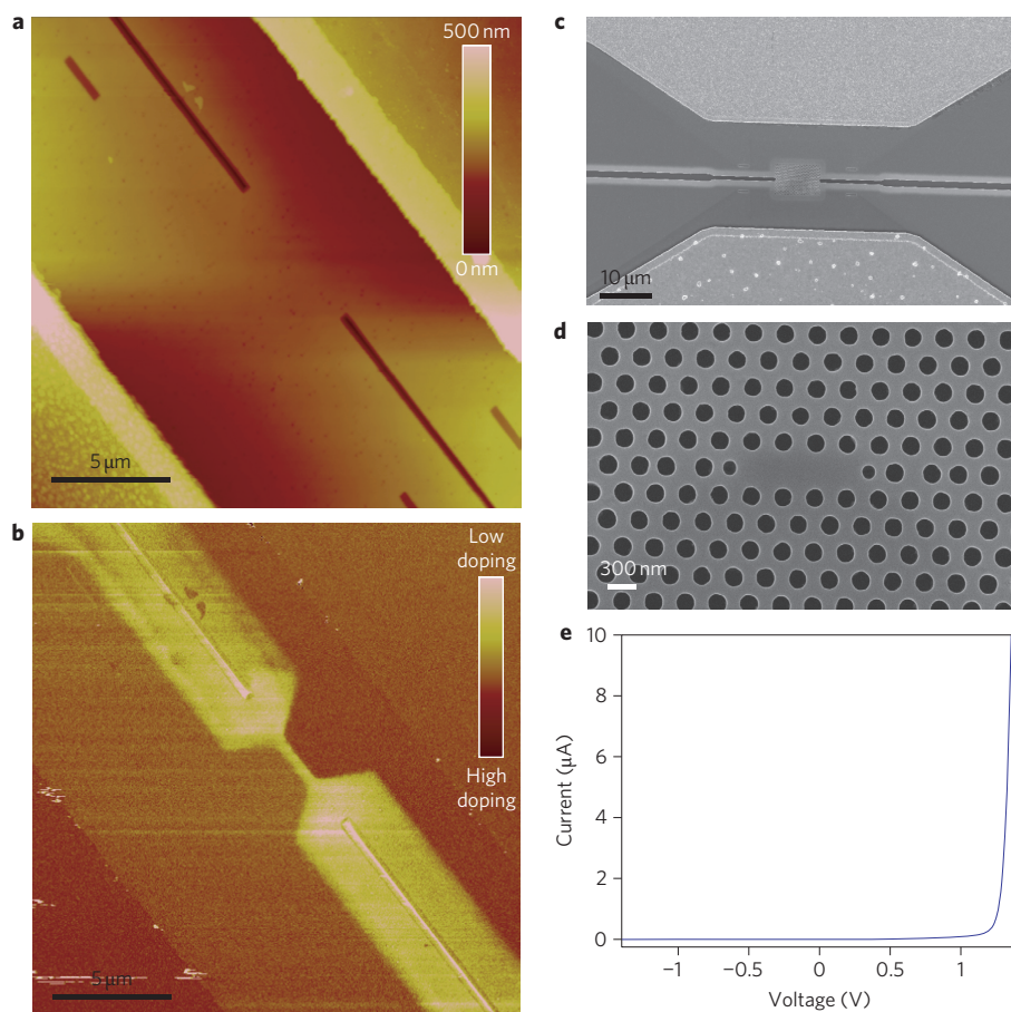
Figure 2 | Fabrication and characterization of the photonic-crystal laser device. a , AFM topography image of the fabricated device without photonic crystal. b , SCM image of the region in a . The p-side of the device is in the lower left corner and the n-side in the upper right. The trench is etched at the device centre, showing the precision of the alignment of the doping regions. 'SCM data' is a combination of the phase and amplitude of capacitance data, where the strength of the signal is directly proportional to the intensity of doping in the local region under the tip. c , SEM image of the fully fabricated laser. The p-side of the device appears on the top of the image, and the n-side on the bottom. d , SEM image of the photonic-crystal cavity (zoom-in of the central region of c ). e , Current-voltage characteristics of the laser taken at 50 K in the dark.
