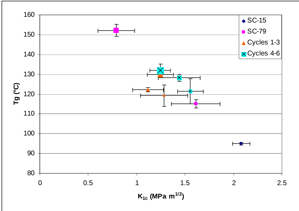
Figure 11. T_g vs. fracture toughness ( K_{1c} ); increasing symbol size corresponds to increasing cycle number.
