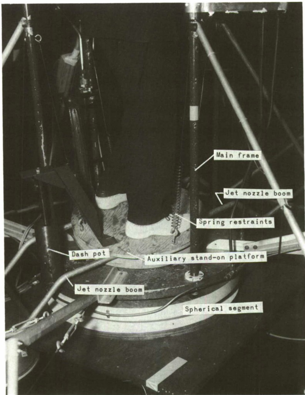
Figure 5.- Auxiliary platform configuration with platform deflected.
