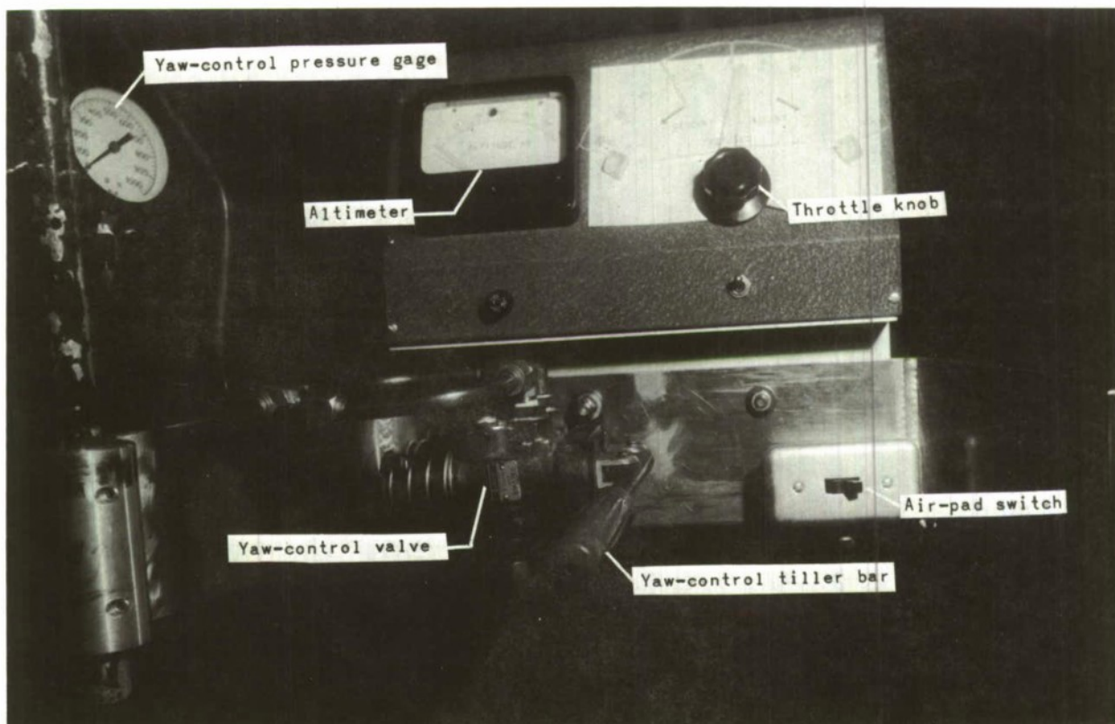
Figure 8.- Control panel.
