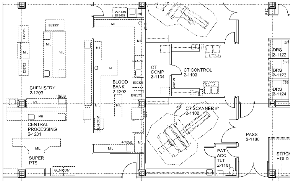
Figure 21. Facility Plan.
