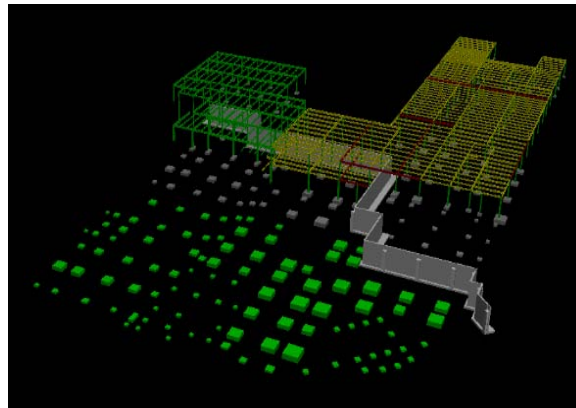
Figure 27. Schedule Simulation.
