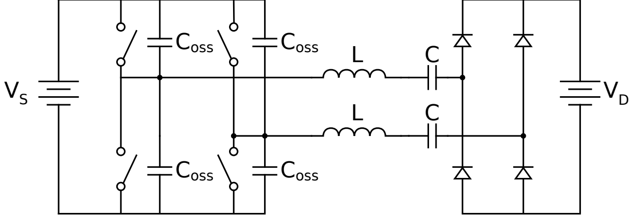
Figure 2: Schematic of a series resonant converter circuit constructed around the coupling capacitors C .
