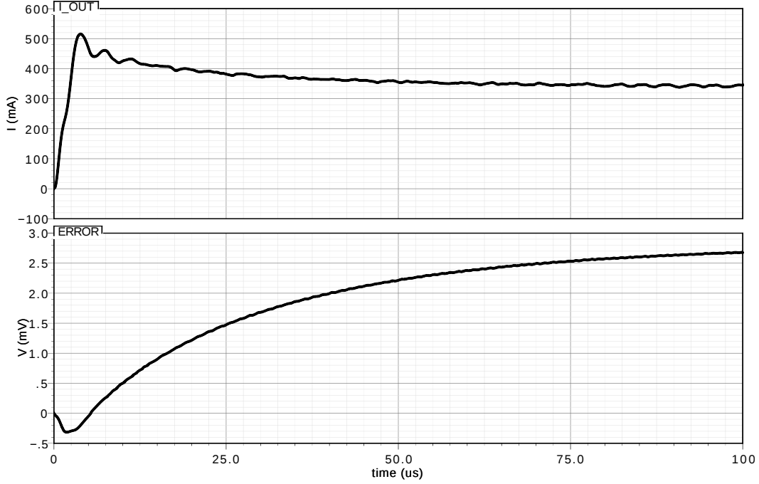
Figure 16: Simulation of current regulation demonstrating loop stability. Top: Output current, I_{OUT} . The final value is 343 mA. Bottom: Error signal; final value 2.8 mV (1 A/V).
