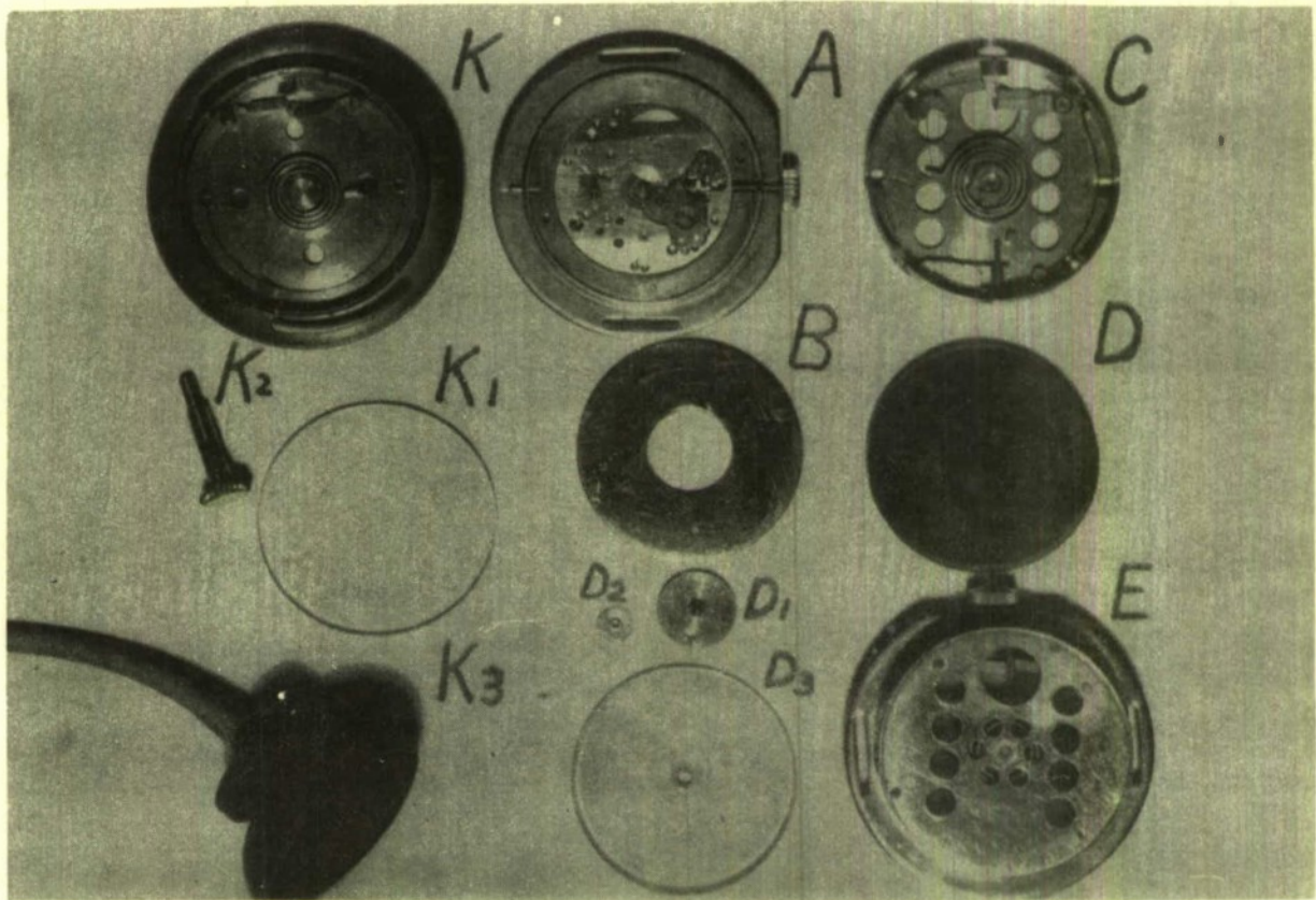
Figure 4 Comparison of the Krogh Micro-Climate Recorder and the C.A.A.-N.R.C. Micro-Recorder (Photographed slightly larger than the actual size)
