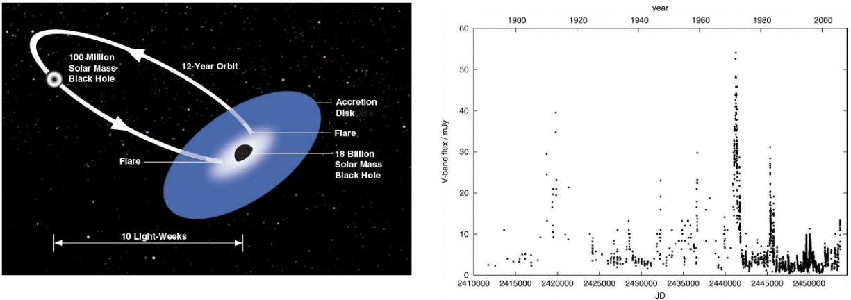
Figure 4a. Artist’s impression of a binary black hole pair in OJ287 (image courtesy Mauri Valtonen, Tuorla Observatory). SIM Lite will be able to track the motion of the suspected binary. Figure 4b. Historical light curve of OJ 287 from Valtonen et al. (2006) showing outbursts at 12 yr intervals. Each outburst is composed of two sharp peaks.
