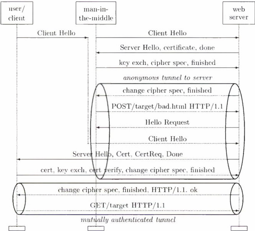
Fig. 2. Man-in-the-middle attack exploiting TLS session renegotiation
