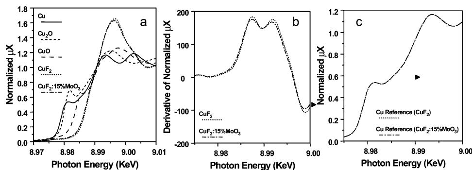
Figure 7. (a) XANES spectra comparing Cu in \text{CuF}_2 :15% \text{MoO}_3 matrices vs that of \text{CuF}_2 and \text{Cu}^{1+} - and \text{Cu}^{2+} -containing oxide standards, (b) derivative of normalized XANES for \text{CuF}_2 and \text{CuF}_2 :15% \text{MoO}_3 , (c) XANES of the reference Cu foil collected simultaneously with \text{CuF}_2 and the \text{CuF}_2 nanocomposite indicating that any small shift observed in the measured spectra is real.
