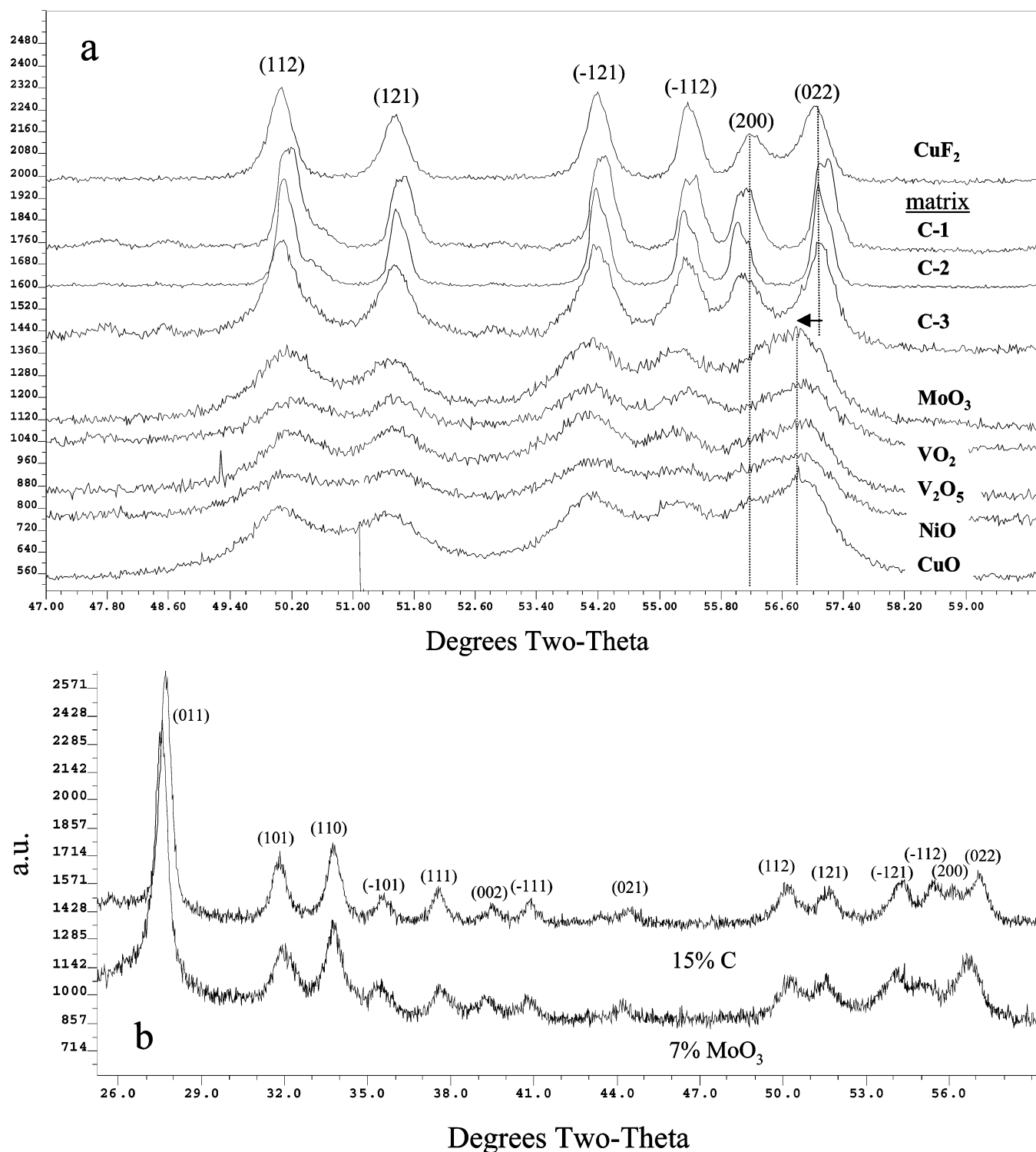
Figure 4. (a) Zoom of the XRD patterns of various nanocomposites vs the CuF 2 standard showing modification of the core CuF 2 structure occurring for all metal-oxide-based matrices. (b) XRD patterns showing contrast in full pattern of a CuF 2 15% C nanocomposite vs a CuF 2 7% MoO 3 nanocomposite leading to expansion of b and c parameters and increase in the \beta angle and volume of the monoclinic structure.
