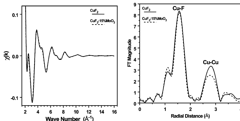
Figure 8. EXAFS spectra (left) and their phase-uncorrected Fourier transform of \text{CuF}_2 :15% \text{MoO}_3 nanocomposite compared with that of the \text{CuF}_2 standard. (FT range 3.0–12.8 \text{\AA}^{-1} , k^3 -weighted, and Hanning window of 1.0 \text{\AA}^{-1} ).
