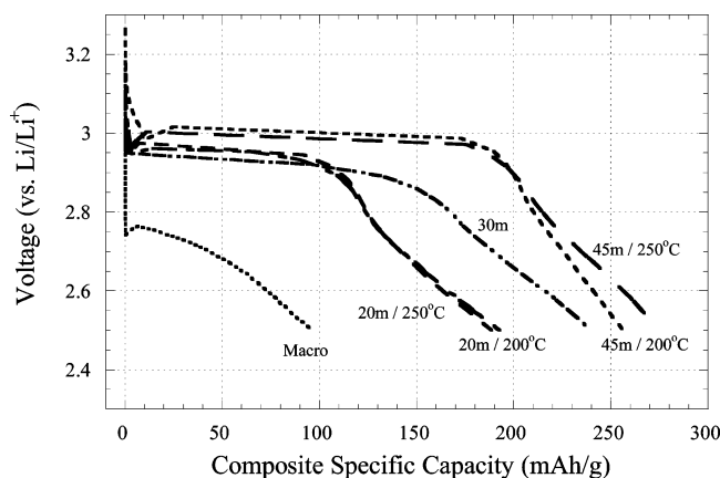
Figure 3. Voltage profiles for 15% C:85% CuF 2 CMFNC nanocomposites of various synthesis parameters. Labels indicate high-energy milling time ( m = min) and postfabrication annealing temperature. All annealing performed for 5 h under He. Macro-CuF 2 mixed thoroughly with 15% carbon is included as reference.
