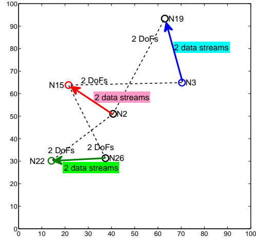
Fig. 6. The DoF allocation on band 1 in the optimal solution for the 30-node network.
