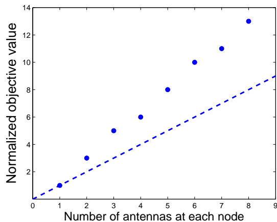
Fig. 7. Normalized objective value under different antennas for the 30-node network.
