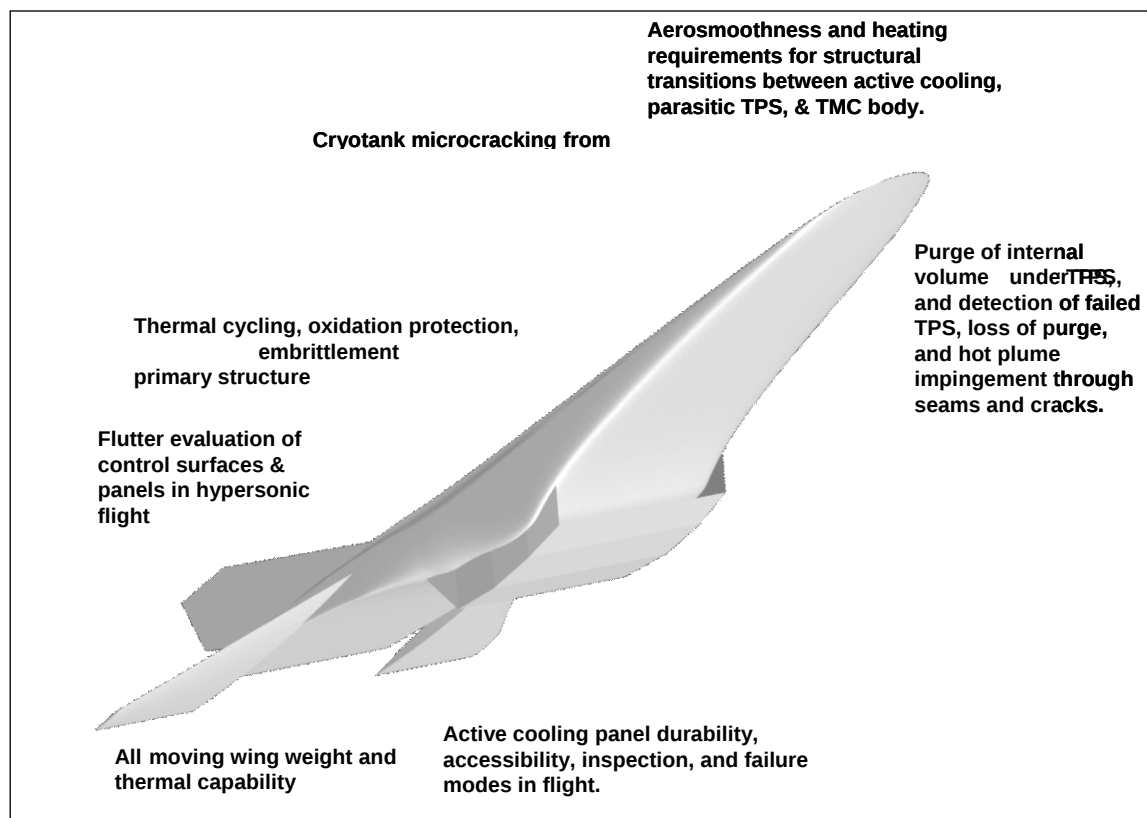
Figure 11. NASP Structural Areas of Concern
