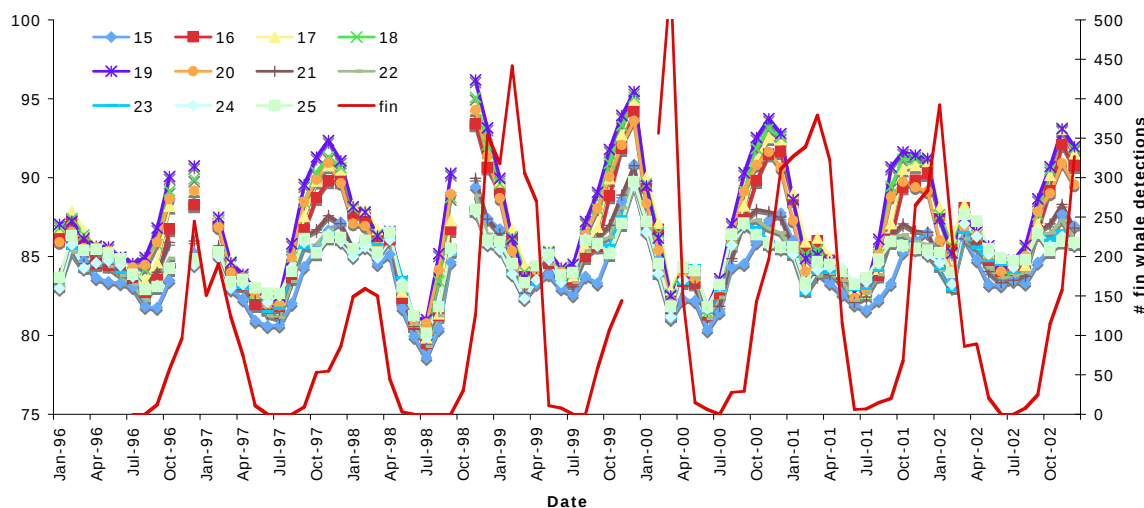
Figure 23. Fin whale detections (solid red line) and relative sound levels for 15-25 Hz from spectra derived from Figure 21 for site O.
