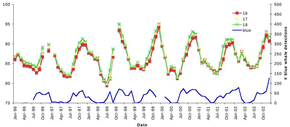
Figure 22. Eastern Pacific blue whale detections (solid blue line) and relative sound levels for 16-18 Hz from spectra derived from Figure 21 for site O.
