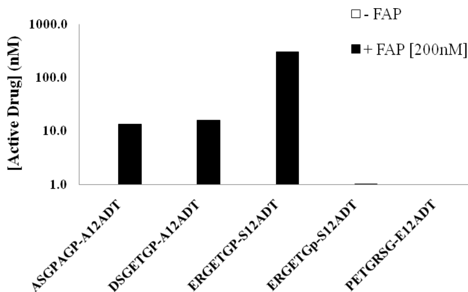
Figure 1: Release of Active Drug (A/S12ADT) from FAP Prodrugs by FAP's enzymatic activity Prodrugs ([100 \mu M]) were incubated with [200nM] FAP at 37 ^{\circ} C for 24h. Aliquots were taken at the indicated time points and concentration of free drug (A/S12ADT) was determined by LC/MS. D-isomer proline represented by 'p'.
