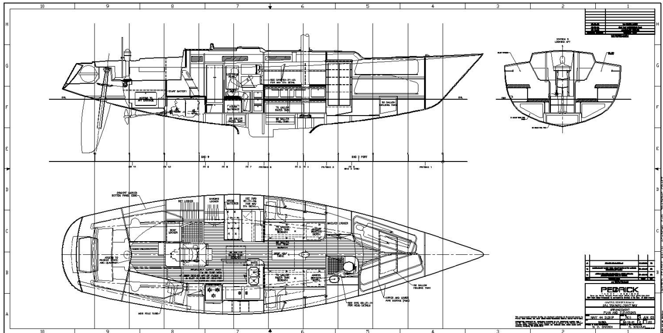
Figure 7: General Arrangement
