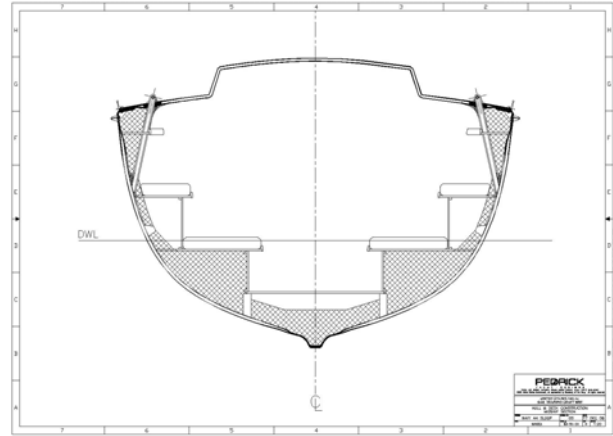
Figure 12: Midships Section
