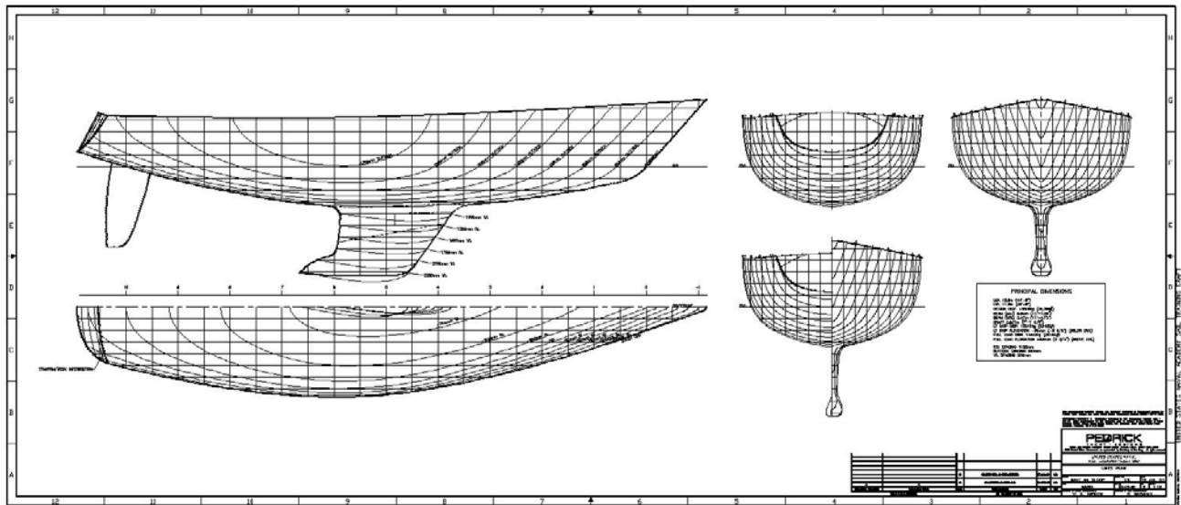
Figure 5: Navy 44 Mk 2 Lines Plan
