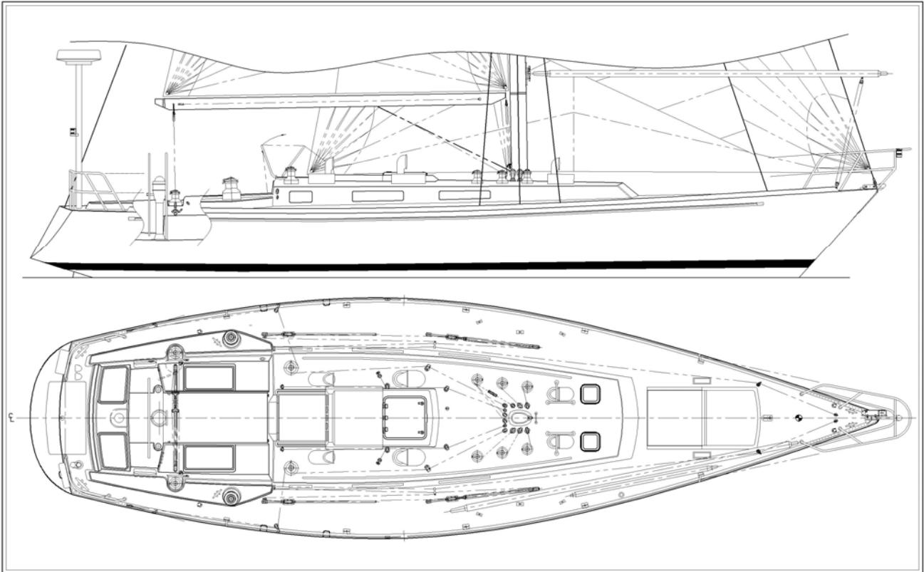
Figure 8: Deck Plan
