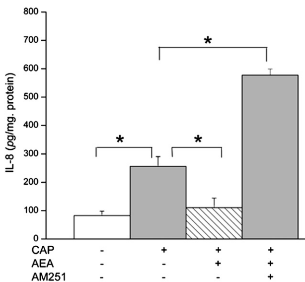
Fig. 9. CB1 activation eliminates TRPV1-induced increases in IL-8 release. HCEC were pretreated with anandamide (AEA; 10 \mu M) and/or AM251 (5 \mu M) for 1 h and then incubated with capsaicin (CAP; 10 \mu M). At the end of the incubation period, the levels of IL-8 were determined by ELISA. The data represent the means \pm SEM ( n = 3 , *P < 0.01 ).
