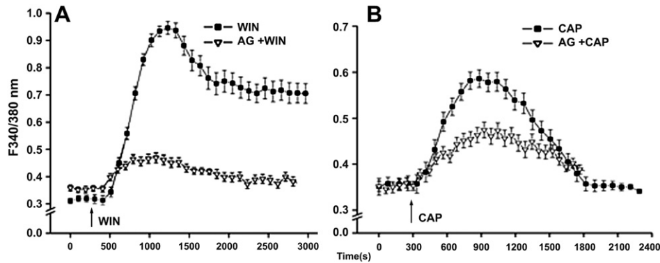
Fig. 3. CB1 and TRPV1 mediate EGFR transactivation. (A) WIN55,212-2 (WIN; 10 \mu M) induced [Ca^{2+}]_i transients in the presence and absence of AG1478 (5 \mu M). (B) Similarly, capsaicin (CAP; 10 \mu M) induced [Ca^{2+}]_i transients in the presence and absence of AG1478 (5 \mu M). The data represent the means \pm SEM ( n = 3 , P < 0.05 ).
