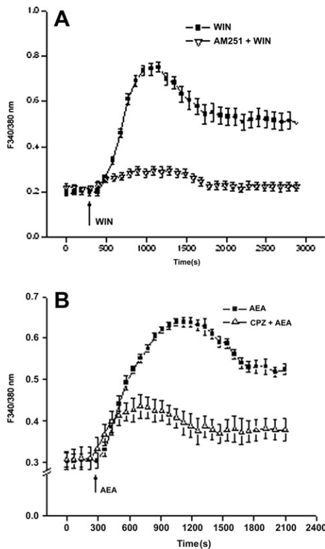
Fig. 2. CB1 functional expression in HCEC. (A) HCEC were loaded with fura2-AM (2 μM). WIN55,212-2 (WIN, 10 μM) induced [\text{Ca}^{2+}]_i transient whereas preincubation with AM251 (10 μM) blocked CB1 activation by 95%. (B) Anandamide (AEA), induced a [\text{Ca}^{2+}]_i transient. Following exposure to 10 μM capsazepine (CPZ) this response was suppressed. The data represent the means \pm SEM ( n = 3 , P < 0.05 ).
