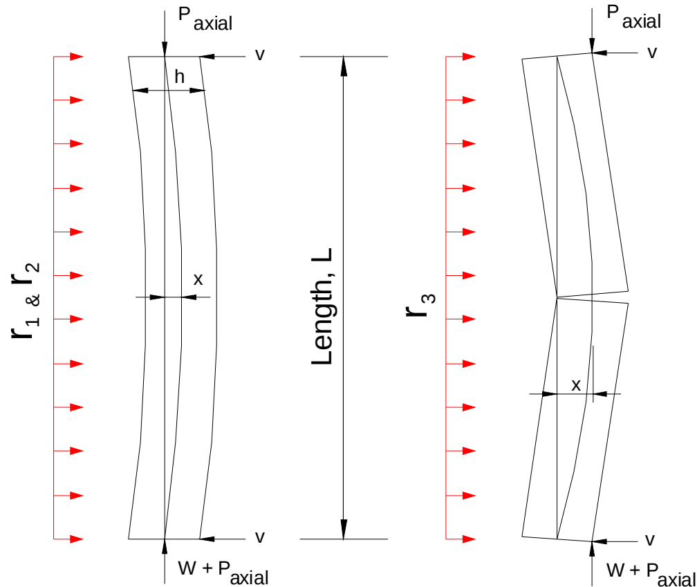
Brittle Flexure
