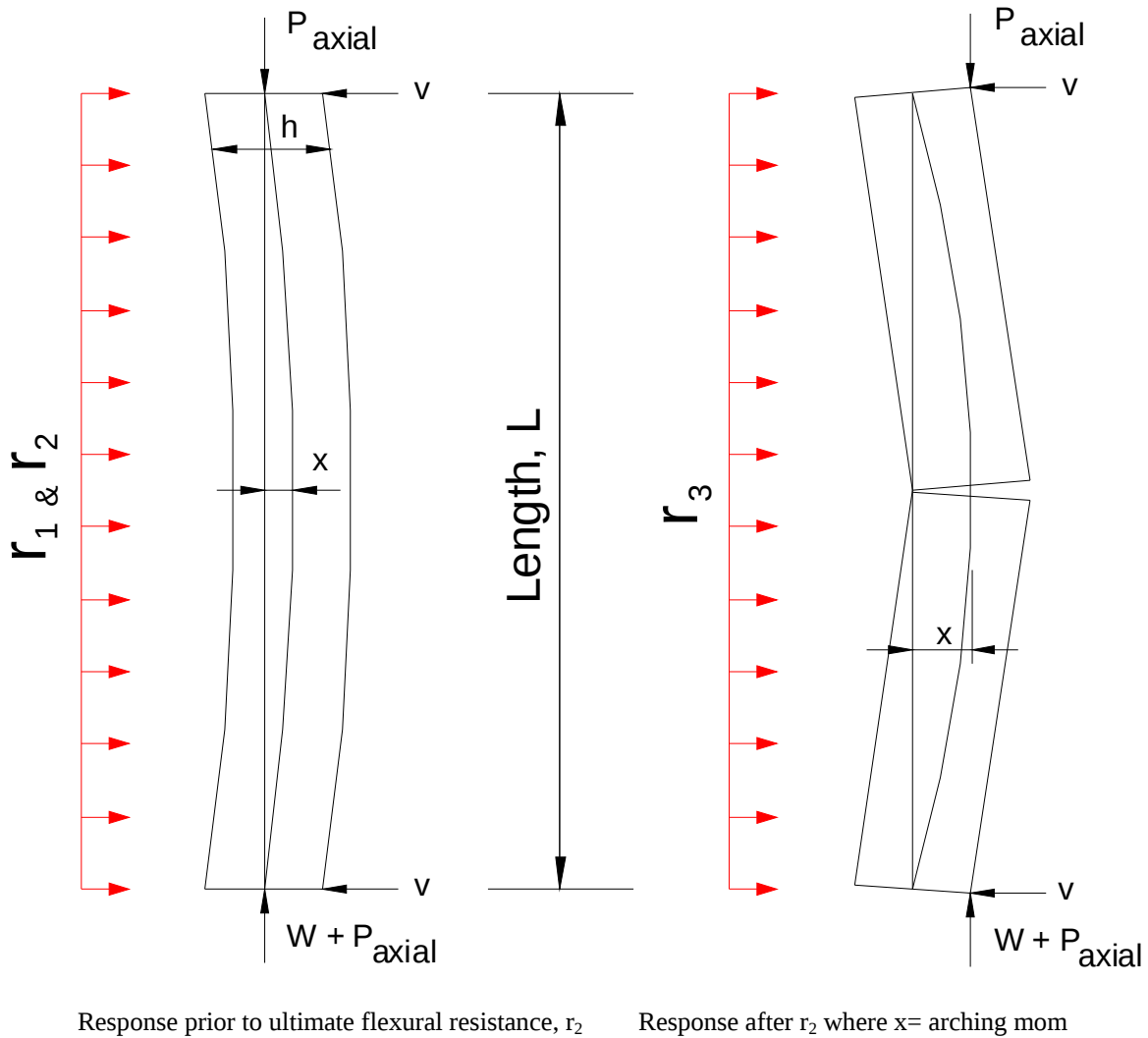
Figure 3. Axial Load Arching in Unreinforced Masonry Walls
