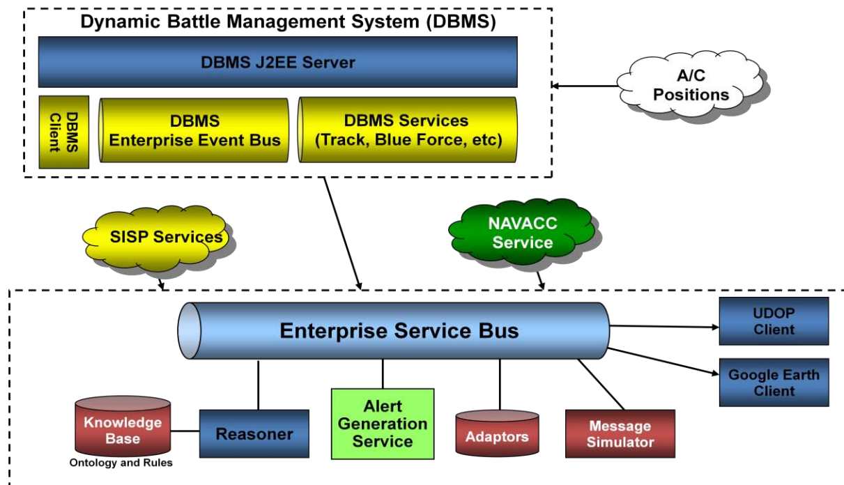
Fig. 1. GSEIS Service-Oriented Architecture
