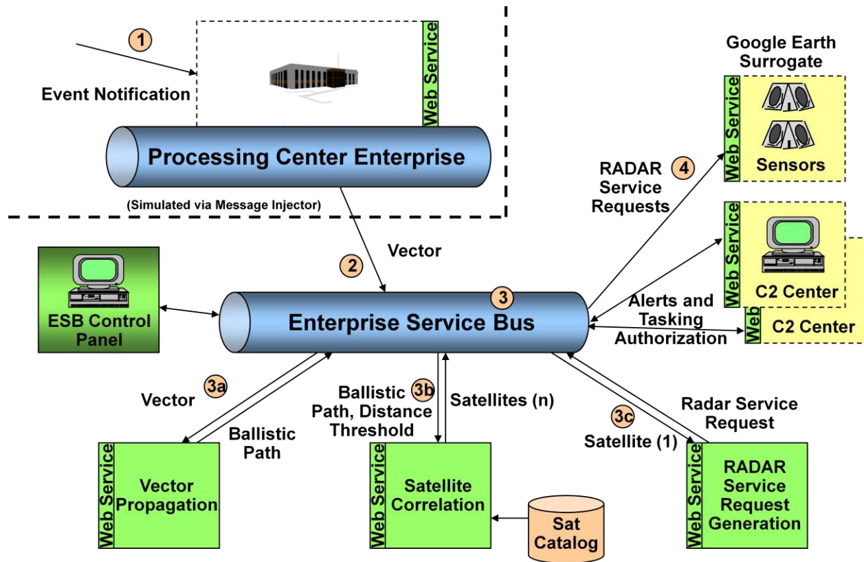
Fig. 2. SOA Reused for Rapid Sensor Tasking
