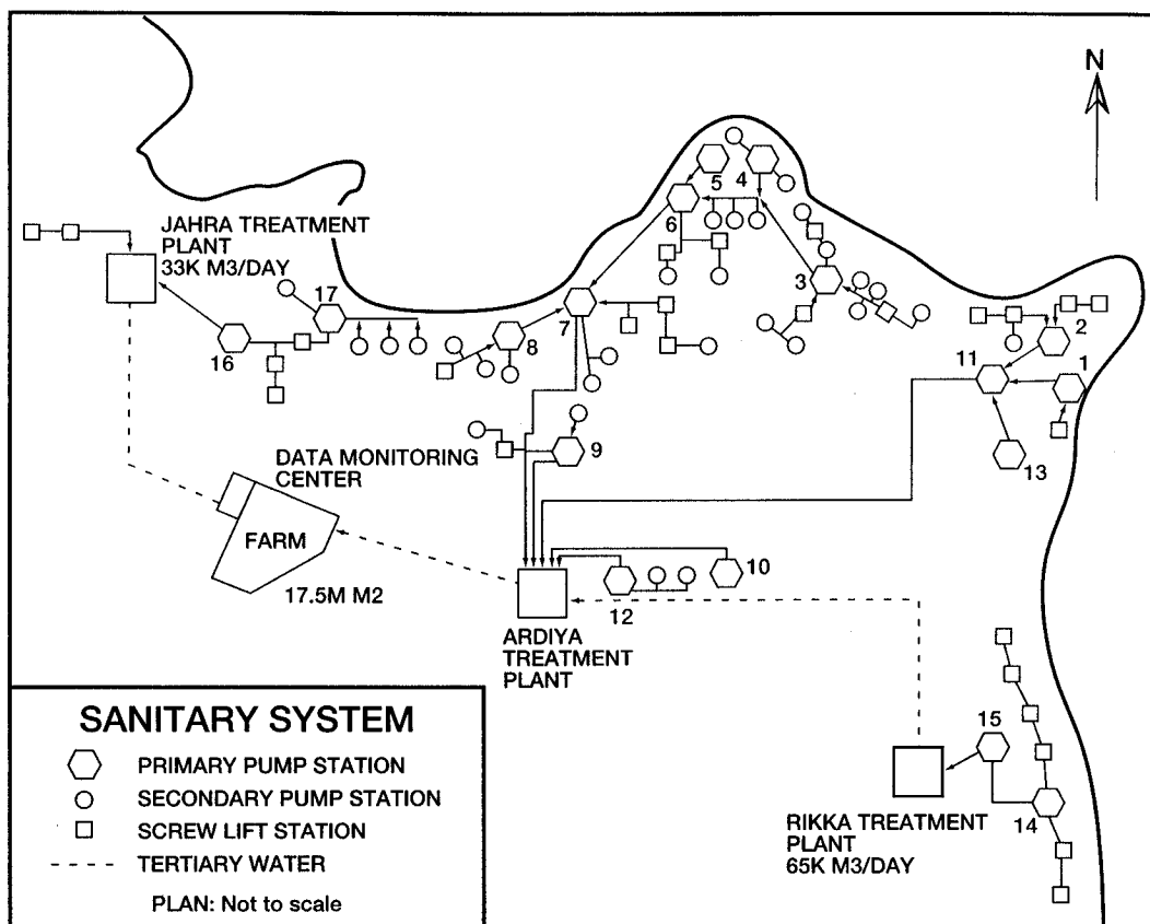
Figure 4—Sanitary System
