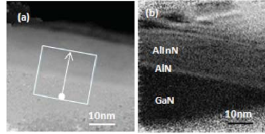
FIG. 3. (Color online) (a) Phase and (b) amplitude images from reconstructed hologram of the HEMT structure.
