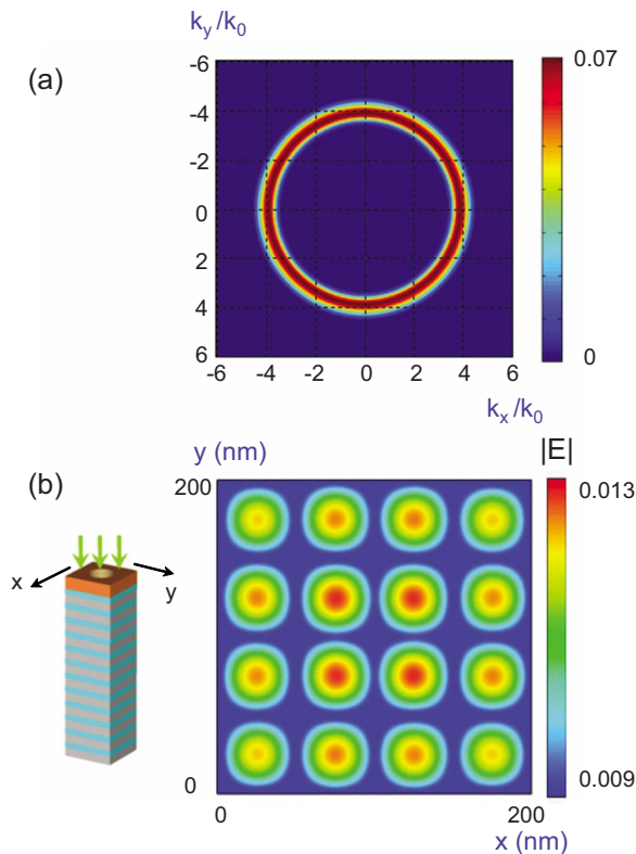
FIG. 3. (Color online) (a) The transmission vs tangential wavevector k_x and k_y (2D transfer function) for a 12 pairs of 35 nm Ag and 21 nm SiO 2 multilayer at a wavelength of 405 nm. (b) The simulated |E| field at the plane 3 nm after the Ag and SiO 2 multilayer. The left inset is the configuration for photolithography. Only one period (200 nm) is shown.
