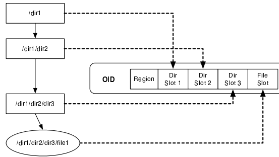
Figure 4.1: File and directory slots. An example file system path and OID are shown. The OID is segmented into a number of directory slots and a file slot. The least significant bits of the OID are to the right and the most significant are to the left. The correspondence between elements in the path and slots in the OID are shown by dotted lines for the child-closest policy.
