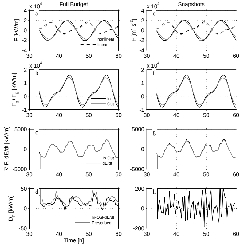
Figure 10: As for figure 9 except for the overturning-based dissipation proposed here. Again, note that d) and h) are different scales.
