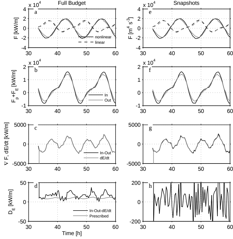
Figure 9: Time series of energy budget for a volume between x = \pm 70 km using constant A_z = 10^{-2} \text{ m}^2 \text{ s}^{-1} . a–d) are using a full budget diagnosed at every time step of the simulation, while e–h) is the same budget from snapshots taken every 20 minutes (37 times a tidal period). a) and e) are the linear (dashed) and non-linear (solid) energy fluxes, the two lines representing the in- and out-going fluxes. b) and f) is the total flux. c) and g) are the flux divergences compared to the rate of change of energy in the volume; these two values lie almost one atop the other. d) and h) is the difference between the energy flux divergence and the energy change in the volume (solid) compared with the prescribed dissipation (gray). Note the difference in scale between d) and h).
