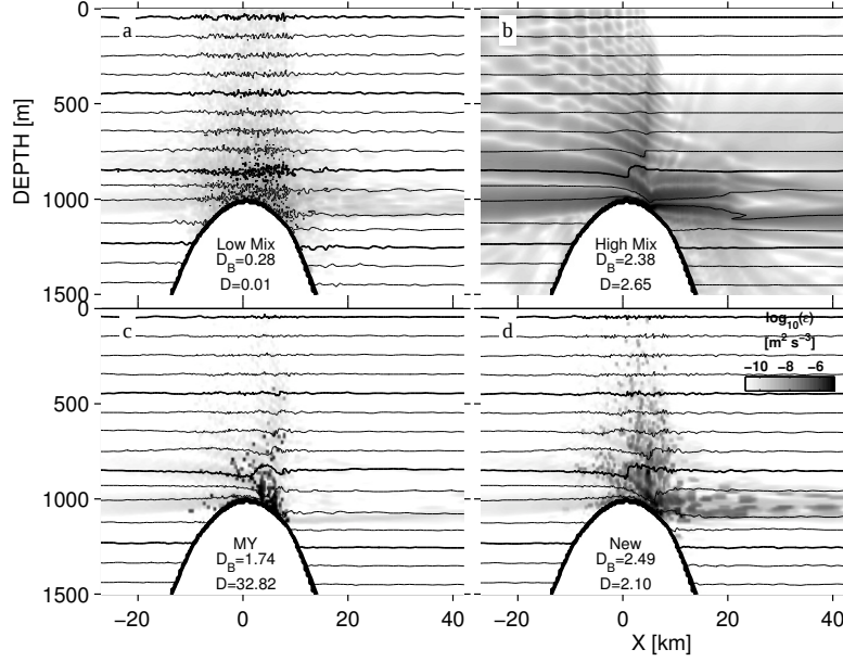
Figure 4: Example dissipation in model runs with steady stratified flow over a large obstacle. The totals are area-integrated dissipation ( [\text{m}^4 \text{s}^{-3}] ) with D_B the difference in the Bernoulli flux past x = \pm 25 km, and D the reported dissipation.
