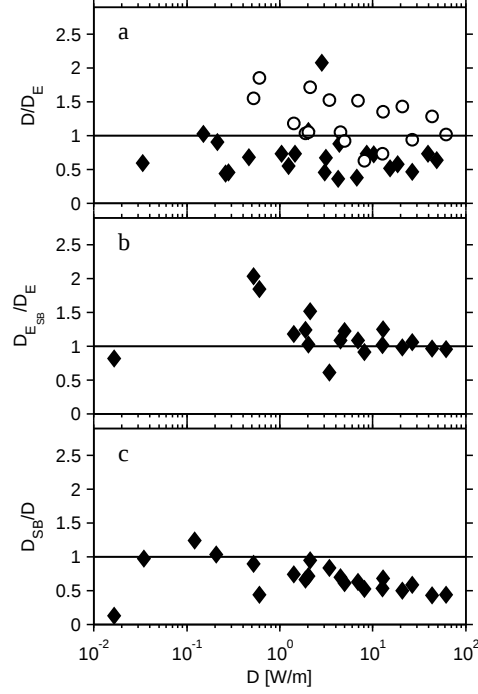
Figure 15: Dependence of dissipation on advection scheme for 10-m resolution oscillating flow over an obstacle: a) dissipation compared with energy divergence for 2nd-order scheme (circles) and superbee advection scheme (diamonds). The superbee scheme tends to have some of its dissipation go unreported, the 2-nd order scheme over-reports its dissipation. b) the ratio of energy divergences in the models. Both schemes lose approximately the same amount of energy except at low dissipations where the superbee scheme dissipates more. c) Because it under-reports, the superbee scheme has less dissipation than the 2-nd order scheme.
