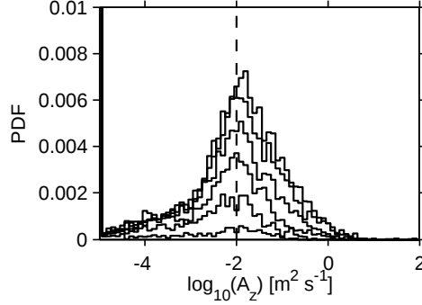
Figure 7: Distribution functions of A_z for the New mixing scheme for the steady flow over an obstacle case, with increasing flow velocities.
