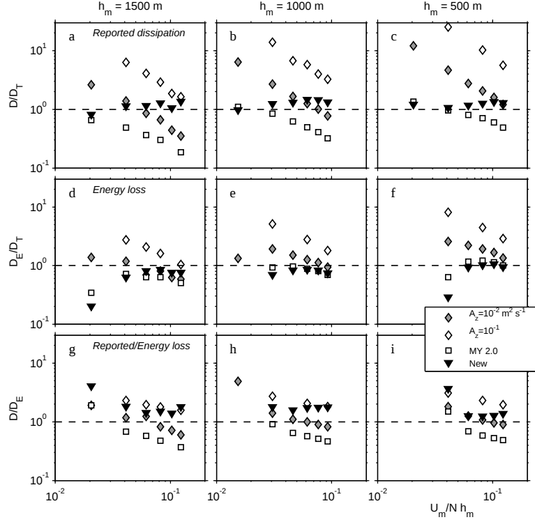
Figure 11: Dissipation in tidal runs for different mixing schemes: a–c) dissipation reported by the viscosity D , compared to a theoretical estimate of the dissipation D_T . d–f) dissipation calculated from an energy budget D_E . g–i) The ratio of reported dissipation to diagnosed dissipation: D/D_E .
