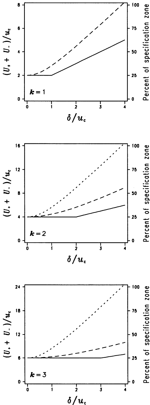
Fig. 5. Comparison of uncertainty interval lengths for three methods of incorporating uncorrected bias in uncertainty intervals. The methods are the proposed SUMU method (solid line), the RSSu_c method (dotted line) and the RSSU method (dashed line). The scale on the right-hand axis of the plots assumes that the value of the expanded uncertainty represents a gauging ratio of 4:1 in the case of zero bias ( \delta = 0 ). (In the case k = 1 , RSSu_c = RSSU .)
