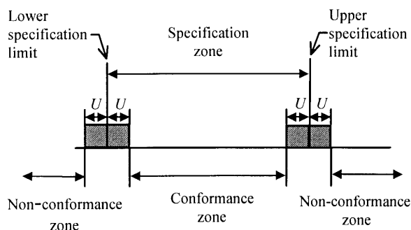
Fig. 1. The functional specification of a part and the corresponding inspection zones; U is the expanded uncertainty of the measurement. Parts are accepted if the measurement result is within the conformance zone.
