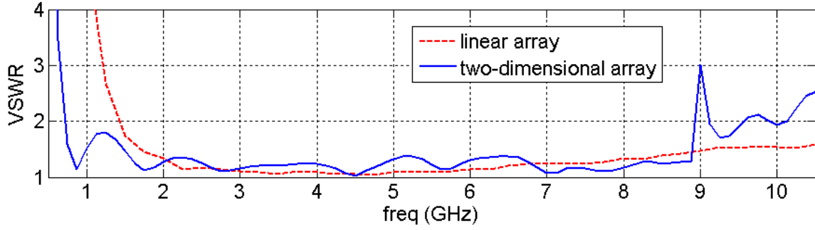
Fig. 9. Comparing the VSWR at broadside radiation for the all-metal element in a linear array versus a two-dimensional planar array; the lack of coupling in the H-plane limits the low-end bandwidth of the linear design.
