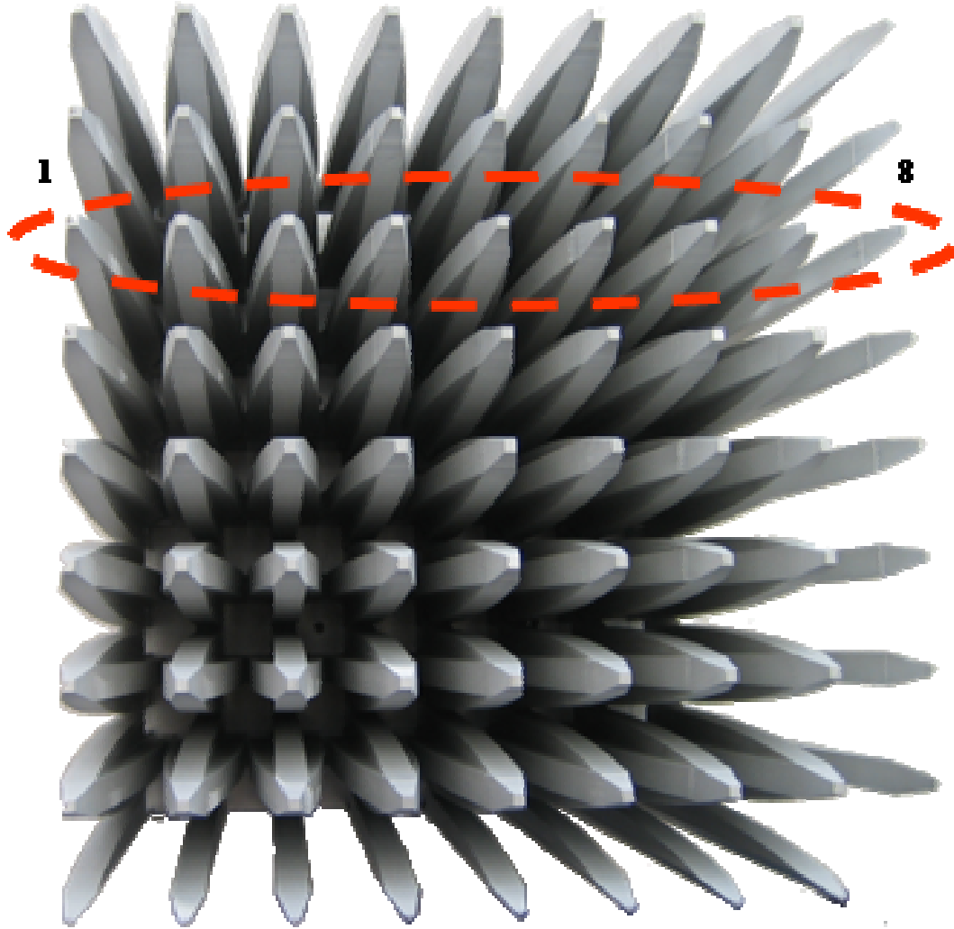
Fig. 13. Top view of the 8x8 dual-polarized flared-notch array. Circled is row number 6 (with numbering) upon which the S-parameter synthesis measurements were performed.
