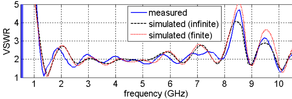
Fig. 11. Active VSWR of element 16 in 32-element linear array element, scanned to positive 45 degrees in E-plane; comparison of measured data, infinite array solution, and exact finite simulation. Simulations and measurements track very well under scan.
