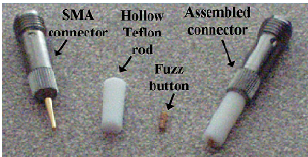
Fig. 4. Design of the element feed for direct coax-to-slot-line transition without soldering. The long outer body of the coax features a knurl that is press-fit into place. The center pin of the coax is extended with a conductive spring-like cylinder (fuzz-button) that achieves contact with the far wall of the antenna slot-line when fully embedded (see Fig. 1 for placement).
