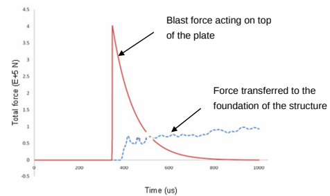
Figure 14: Blast loading versus reaction force on the vehicle.
