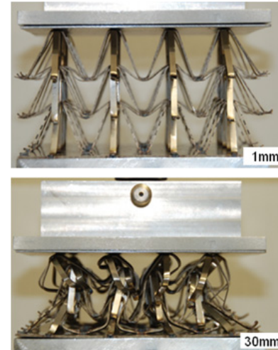
a) Experimental setup and deformation of the NPR sample under a quasi-static compressive load
