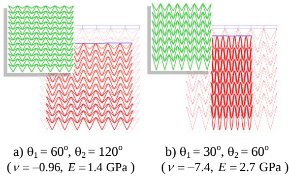
Figure 3: Two example NPR material samples.
