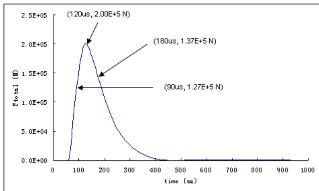
b) Blast loading history
