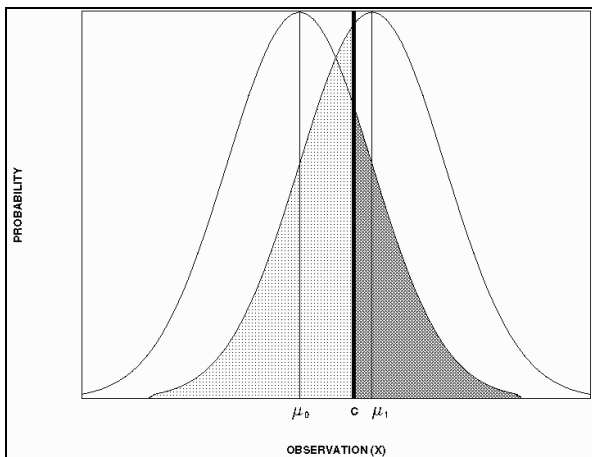
Figure 3: Normal Distributions.
