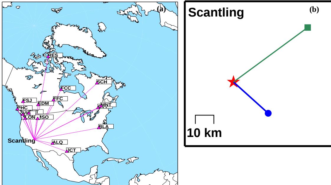
Figure 6. Nuclear explosion Scantling, 19 August 1977. Figure (a) depicts the azimuthal distribution for the network and their great circle path to the actual location for the explosion used to determine the epicenter by P-wave arrival times and Rayleigh waves maximum spectral energy arrival times. Figure (b) depicts the mislocation vectors for the determined epicenters. ★ shows the actual location, ■ shows the P-wave location, and ● shows the Rayleigh wave location. Here the location error for P-wave is 49.9 km and for Rayleigh MSE is 25.1 km.
