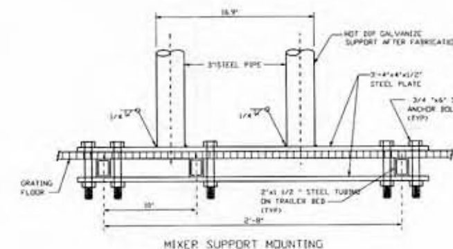
MIXER SUPPORT MOUNTING
