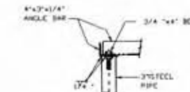
DETAIL C
