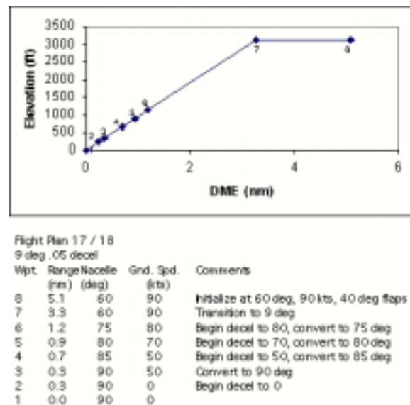
Fig. 13. Flight Plan 17, 9 degree 0.05 g decelerating approach.
