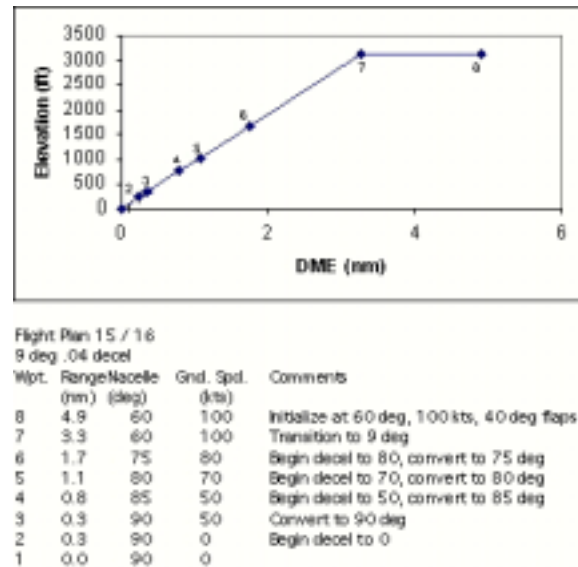
Fig. 12. Flight Plan 15, 9 degree 0.04 g decelerating approach.
