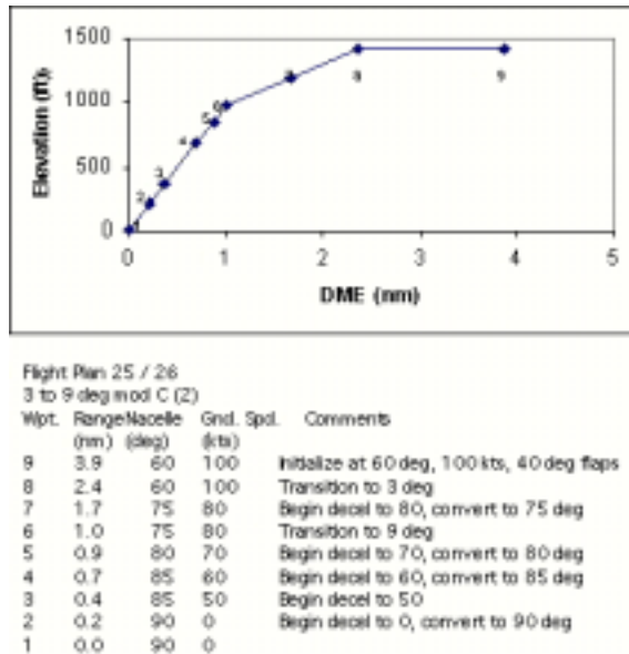
Fig. 10. Flight Plan 25, 3-9 degree double segment approach.
