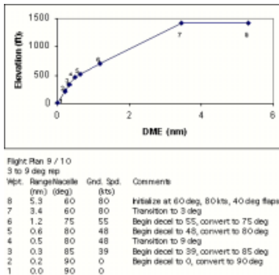
Fig. 11. Flight Plan 9, 3-9 degree approach used with 40 and 75 degree maximum flap use investigation.
