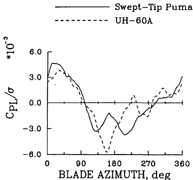
Figure 3. Comparison of pitch-link load measurements with azimuth from the swept-tip Puma and UH-60A; \mu = 0.362 and C_T/\sigma = 0.070 (Flight 525) for the Puma and \mu = 0.355 and C_T/\sigma = 0.080 (Flight 9) for the UH-60A; 1-64 harmonics.
