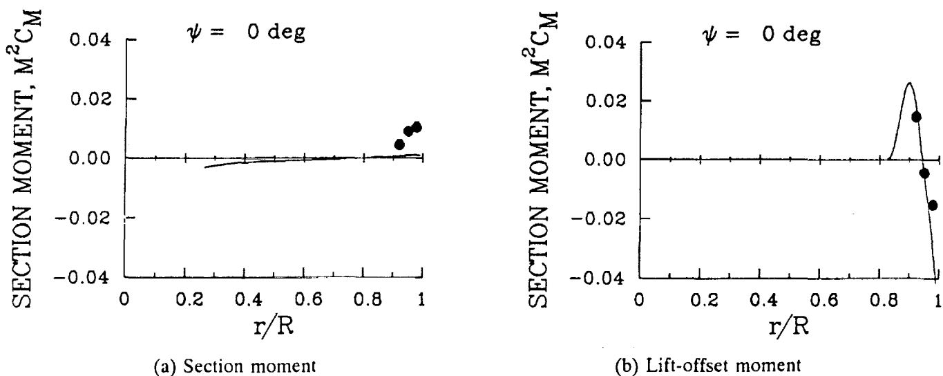
Figure 15. Comparison of CAMRAD/JA prediction and flight test data for aerodynamic section moment and lift-offset moment for the Puma at \psi = 0^\circ ; \mu = 0.402 and C_T/\sigma = 0.070 (Flight 525); 1–64 harmonics.
