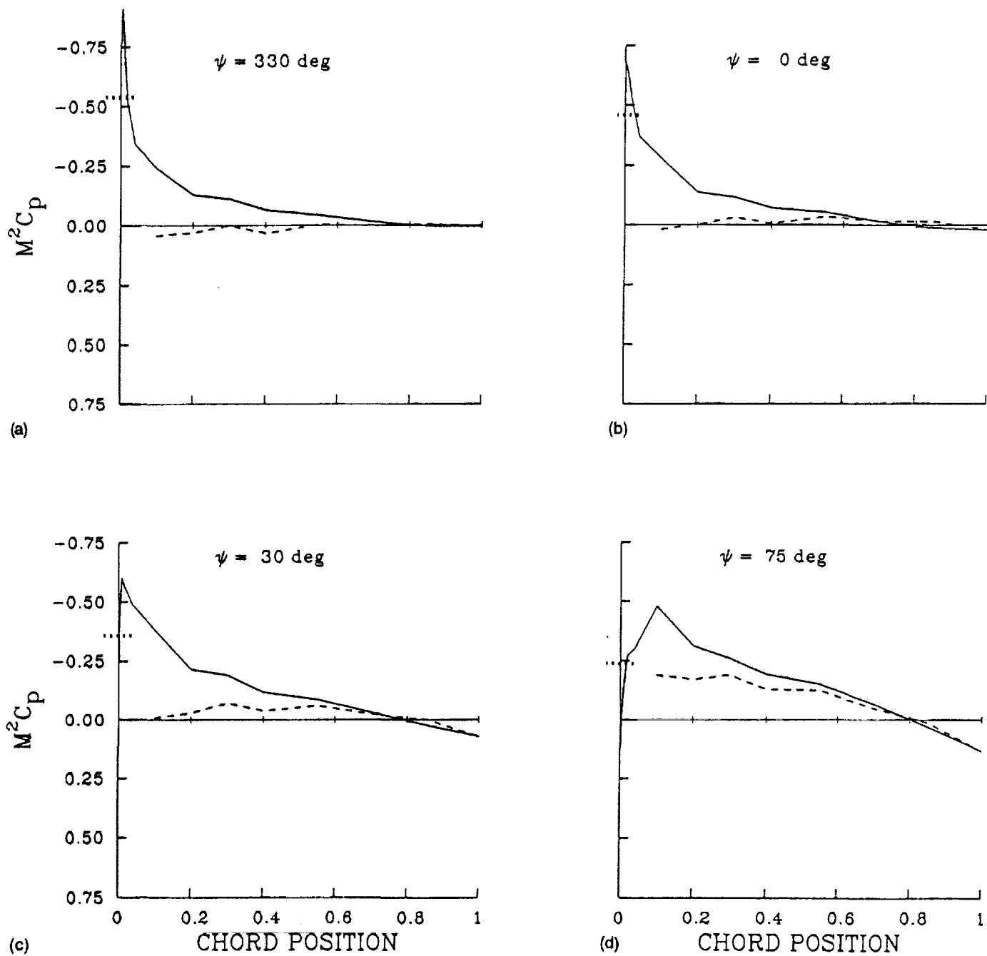
Figure 18. Chordwise pressure distribution for the swept-tip Puma blade through the positive section moment peak; r/R = 0.978 , \mu = 0.376 and C_T/\sigma = 0.080 (Flight 456); 1-64 harmonics.
