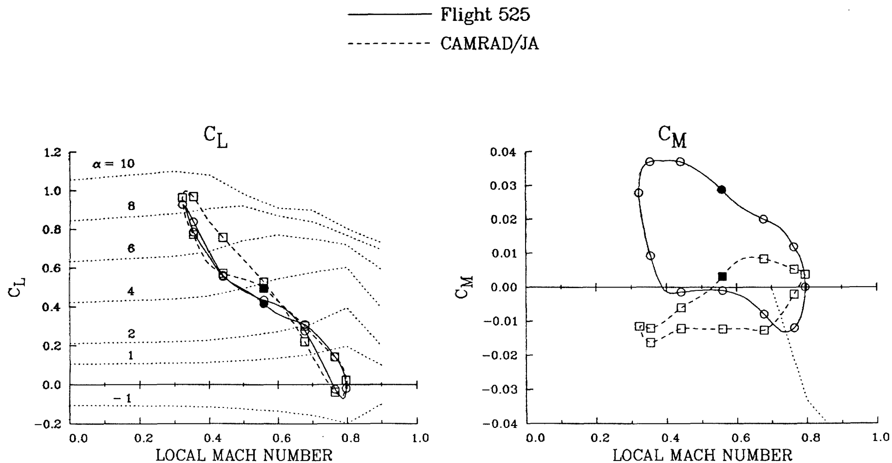
Figure 10. Comparison of predicted and measured aerodynamic section lift and moment as a function of Mach number for the Puma; two-dimensional airfoil data shown as short, dashed line; solid symbols indicate \phi = 0^\circ , open symbols every 30^\circ , r/R = 0.95 , \mu = 0.402 , and C_T/\sigma = 0.070 (Flight 525), 1–12 harmonics. (a) Section lift; (b) section moment.
