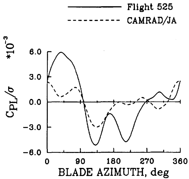
(a) Swept-tip Puma: \mu = 0.402 and C_T/\sigma = 0.070 (Flight 525)
