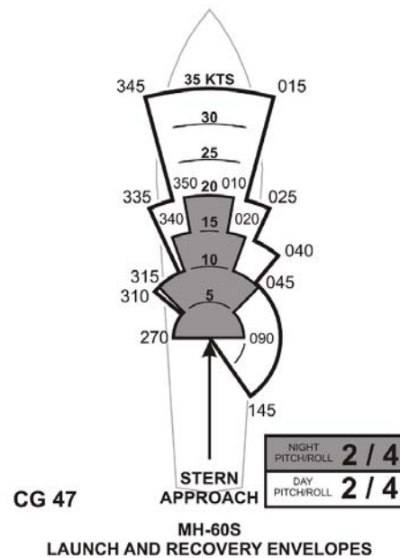
Figure 1. Launch and recovery envelopes for MH-60S helicopters on USS Ticonderoga (CG 47) class cruiser (Ref 1).
