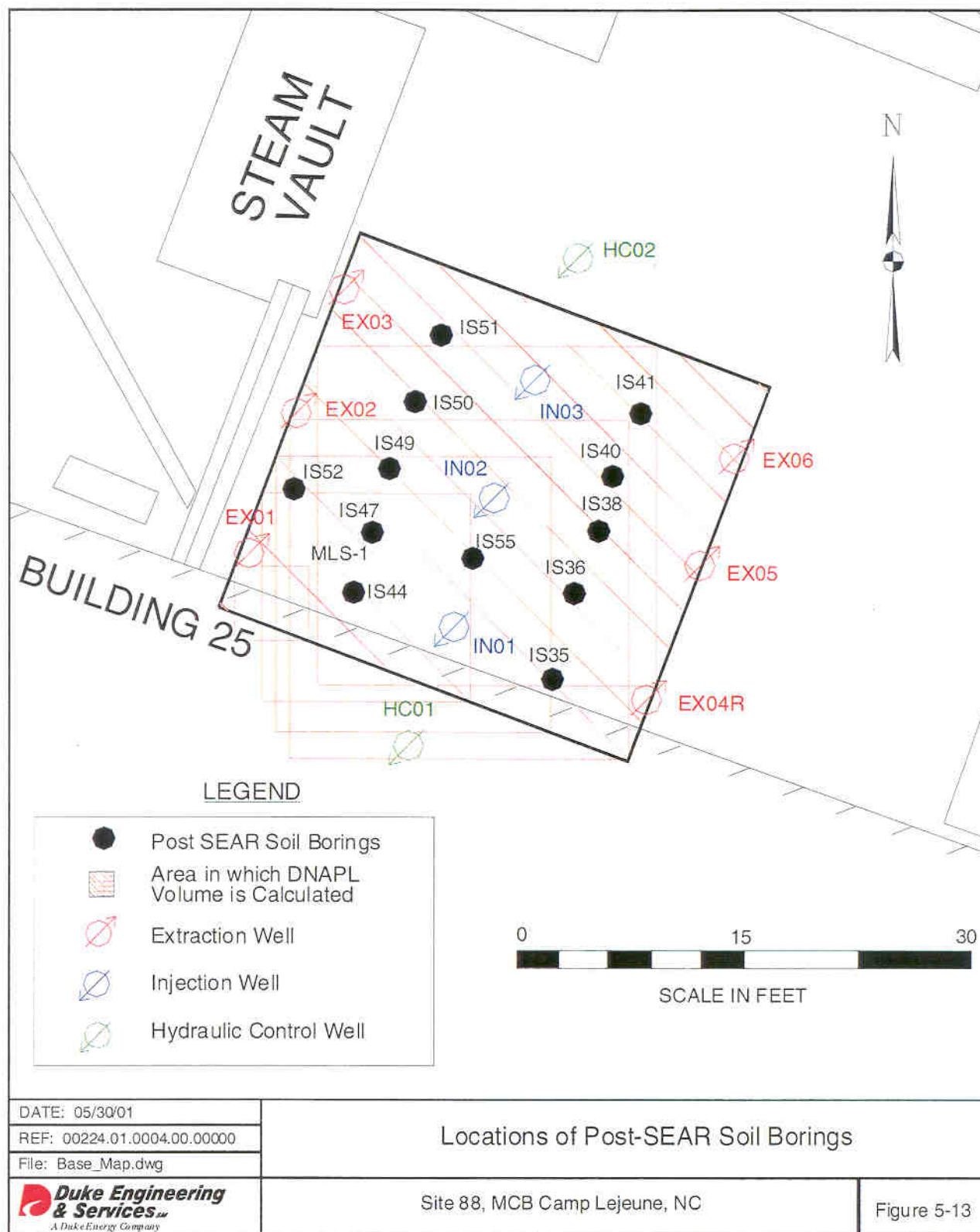
Figure 5-13. Post-SEAR Soil Boring Locations at Site 88, MCB Camp Lejeune, NC
