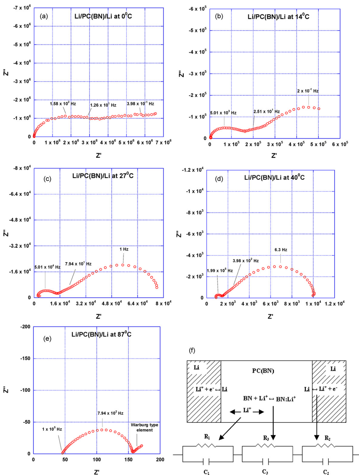
Fig. 6. Nyquist plots of a Li/PC(BN)/Li cell at (a) 0, (b) 14, (c) 27, (d) 40, (e) 87 °C after 552 h of aging at room temperature, and (f) equivalent circuit of a Li/PC(BN)/Li cell.
