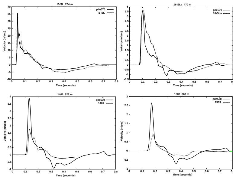
Figure 1. Particle velocity measurements at working point depth from PILEDRIVER compared to numerical simulation pile570 using the effective stress law.
