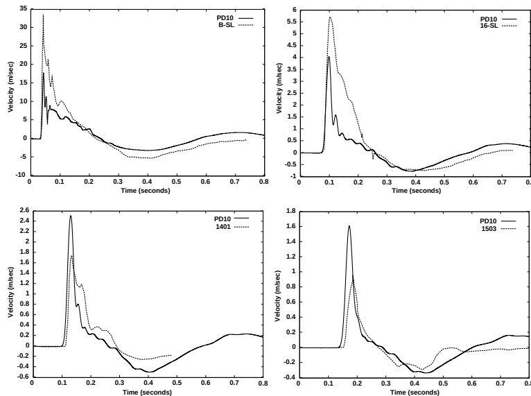
Figure 6. Calculated particle velocity pulses at four ranges for Run PD10 and PILEDRIVER measurements
