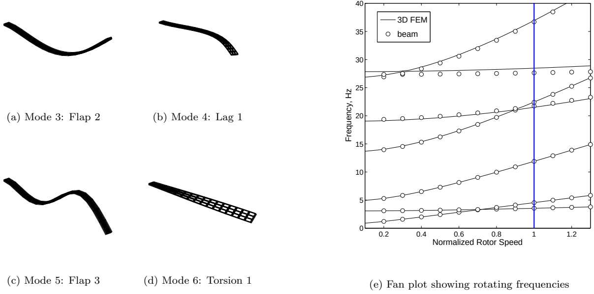
Figure 4: Rotating frequencies and mode shapes of an uniform soft in-plane hingeless rotor of aspect ratio 20, thickness 25% chord; 3-D bricks vs 1-D beam; 16 \times 3 \times 3 grid
