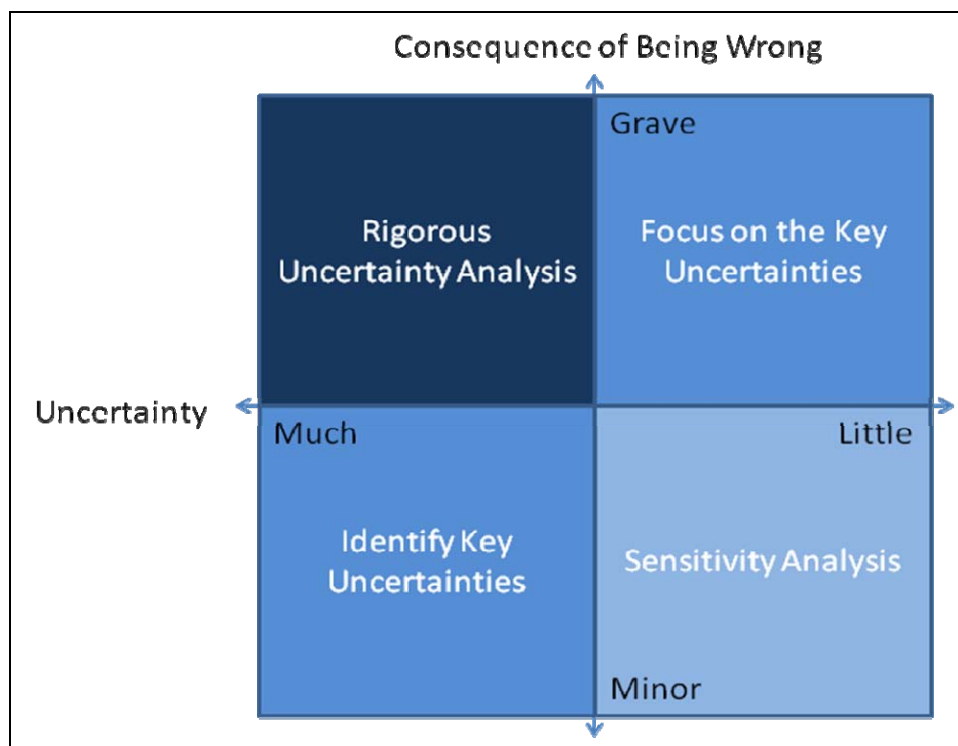
Figure 4. When to perform uncertainty analysis.
