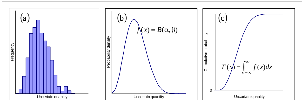
Figure 5. Three ways to describe uncertainty in a random variable. Panel (a) presents a histogram (often used to model empirical data), Panel (b) presents a probability density function (PDF), and Panel (c) presents a cumulative distribution function.
