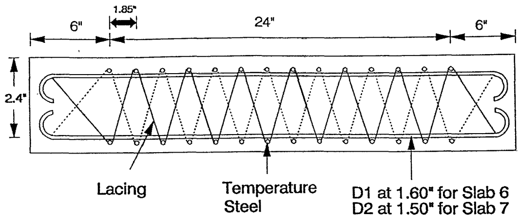
Figure 3. Sectional View Through Length of Slabs No. 6 and 7
