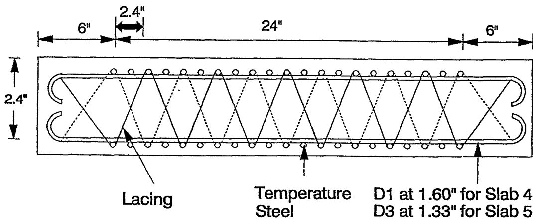
Figure 2. Sectional View Through Length of Slabs No. 4 and 5
