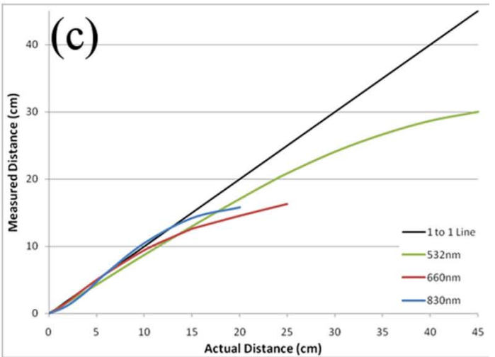
Fig. 6 Actual vs. Measured distance plots comparing all three of the wavelengths tested (black target). In clean water, the performance of lower wavelengths is much better, but as the water becomes more turbid, the performance converges. (a) Clean. (b) Coastal Ocean (c) Turbid Harbor.
