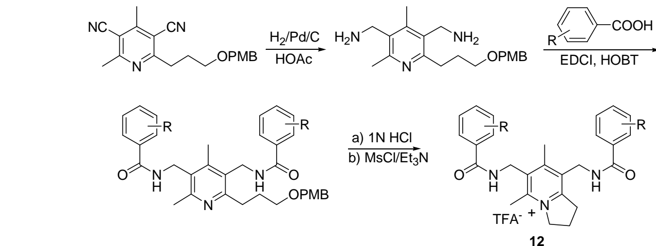
Scheme 4. The chemical synthetic routes to synthesize novel ligands.
