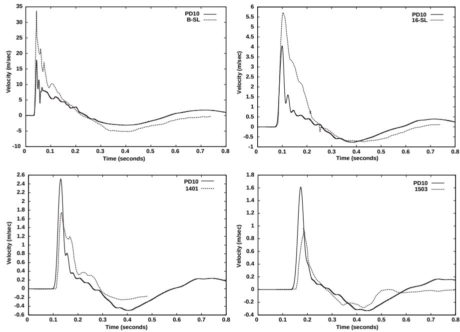
Figure 4. Calculated particle velocity pulses at four ranges for Run PD10 and PILEDRIIVER measurements.
