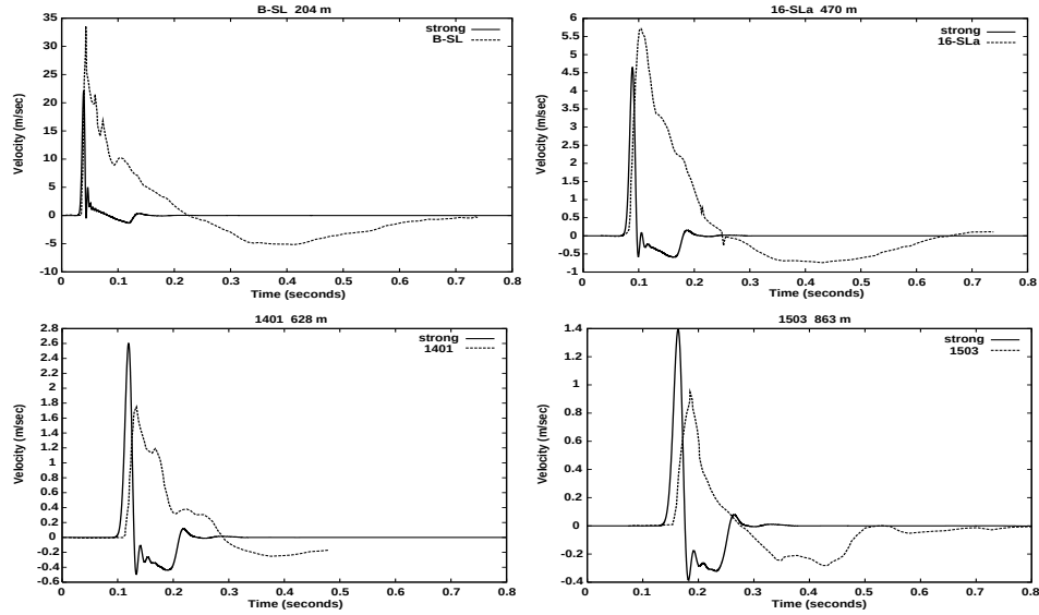
Figure 1. Particle velocity measurements at working point depth from PILEDRIVER compared with data from a calculation using the laboratory strength of granite with no weakening.
