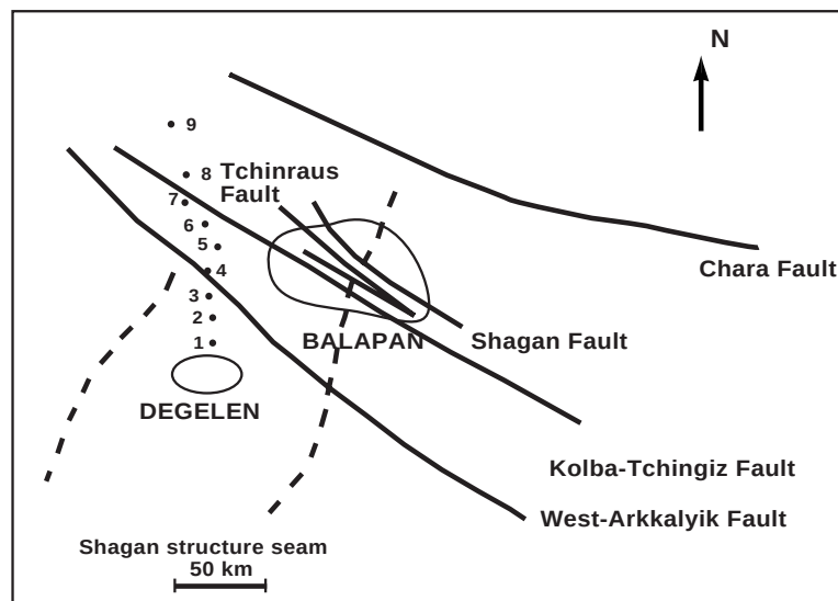
Figure 3. Map showing the locations of the former Soviet Degelen and Balapan test sites, faults, and seismic stations in the region. We will analyze near field waveforms from the Degelen test site, and seismic data recorded at stations 1 through 9 north of the test site for the same events.
