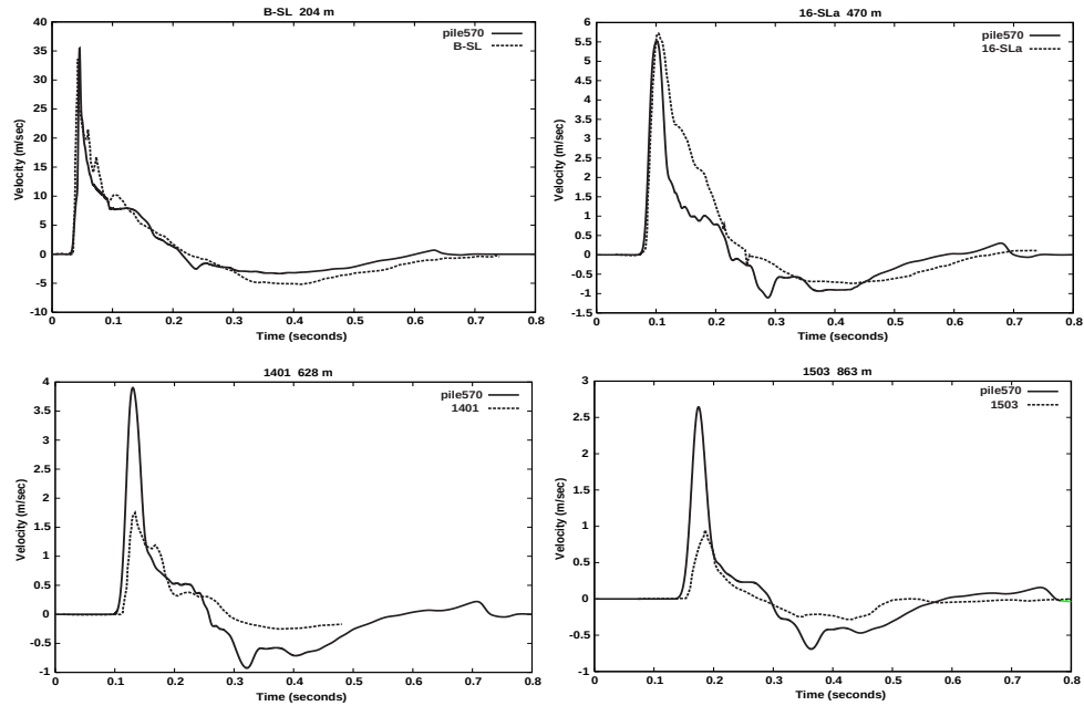
Figure 2. Particle velocity measurements at working point depth from PILEDRIVER compared to numerical simulation pile570 using the effective stress law.
