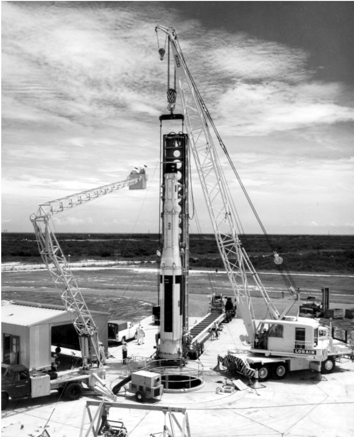
Figure 31. Minuteman I lifted from transporter/erector for lowering into silo (NARA).
