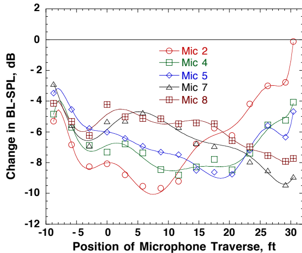
Fig. 18. Changes in advancing side BVI noise with 3^\circ of 2/rev IBC at 190^\circ phase angle for traverse sweep at 75 kts (shaft angle = 4^\circ ).
