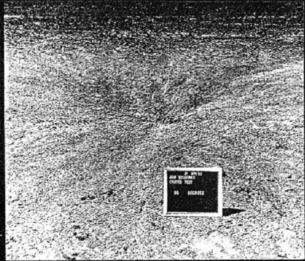
POST-TEST
