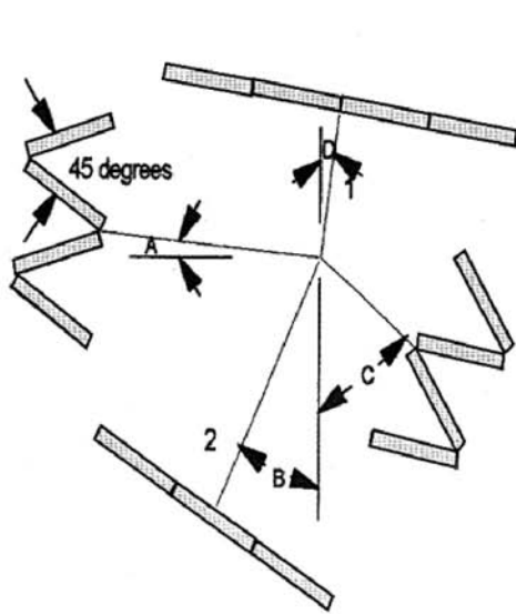
CONCRETE JERSEY BARRIERS
