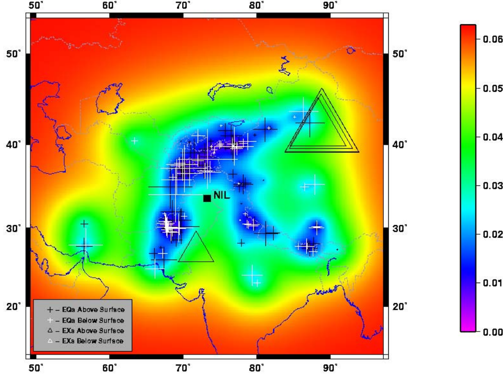
Figure 4. Uncertainty (variance) surface for \log[\text{Pn/Sn}(6\text{--}8 \text{ Hz})] at NIL. Triangles show locations of nuclear explosions and crosses show the locations of earthquakes. The markers are the same as Figure 3.
