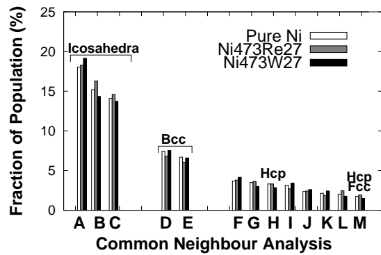
Figure 3: Common Neighbour Analysis of pure Ni, Ni_{473}Re_{27} and Ni_{473}W_{27} at 1830 K. The combined analysis shows the presence of similar short range order in the three samples, with almost no dependence on composition. Icosahedral and bcc-type ordering are found to be the most abundant.
