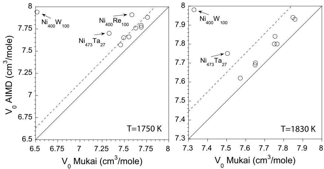
Figure 6: Comparison of molar volumes calculated with AIMD simulations and estimated using the Mukai parametrization. Data in perfect agreement would fall on the line representing a slope of one, the dashed line indicates where the two results differ by 2 percent. The outliers are compositions that fall outside the composition ranges included in the fit of the Mukai model.
