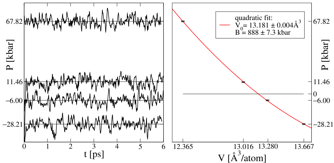
Figure 5: Graphic representation of the equation of state calculations for liquid metal \text{Ni}_{400}\text{Al}_{100} alloy at 1830 K. Representative AIMD calculations of pressure as a function of simulation time for four volumes (left) with a horizontal line indicating time averaged values. The volume at these pressures, with error bars, (right) are fit to a quadratic polynomial, with results of this least squares fit shown in inset. Interpolating to the zero pressure volume produces the predicted equilibrium volume the bulk modulus and it's derivative for a given composition and temperature. Error bars and estimated uncertainties are based on standard uncertainty analysis.
