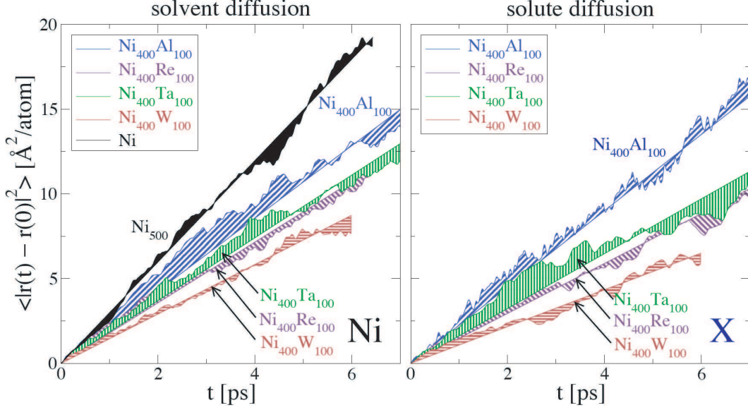
Figure 1: Calculated AIMD mean-square displacements of solvent (left) and solute (right) species for elemental Ni and binary Ni-X (X=Al, W, Re, and Ta) alloys at 1830 K. Deviations in the "random walk" from the long-time linear diffusion relation, \langle |r(t) - r(0)|^2 \rangle = 6Dt , are shown as filled areas for each species. The results shown here are from the lowest pressure simulations at these chemistries. The diffusion constants (D) in Table 1 are derived from the slopes of the mean square displacement curves at several volumes interpolated to zero pressure. Self diffusion of Ni decreases with solute additions with Al producing the smallest effect and W the largest. The relative solute diffusion in these liquid Ni-X metals follows the same trends of the respective solvent diffusion.
