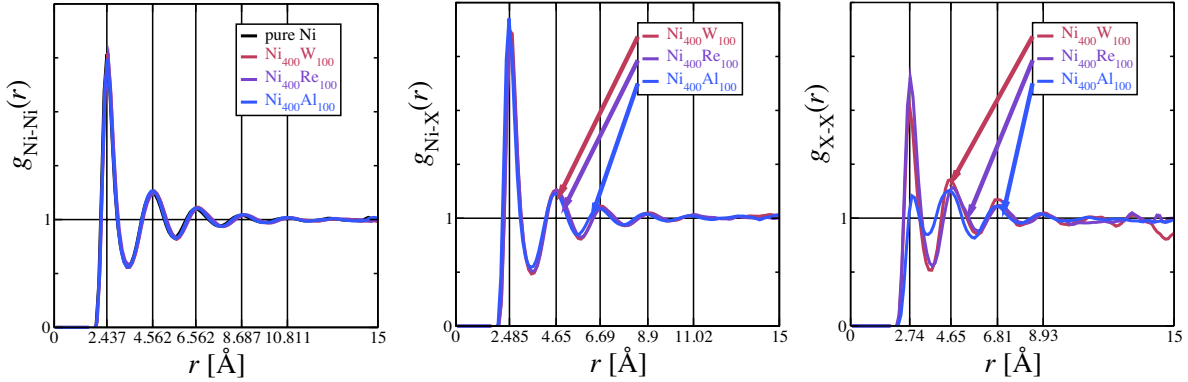
Figure 2: Radial distribution functions calculated from AIMD simulations for elemental Ni and binary Ni-X (X=Al, W and Re) alloys at T=1830 K. The three plots show results, from left to right, for solvent-solvent (Ni-Ni), solvent-solute (Ni-X) and solute-solute (X-X) pairs.
