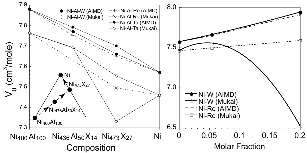
Figure 7: Variation of molar volumes at 1750 K for ternary and binary alloys calculated using AIMD simulations and estimated using the Mukai parametrization. The figure on the left shows compositions spanning the ternary triangle (see inset). Results are linear in composition with deviations from linearity of less than 0.8 %. The Mukai model results for Ni_{473}Ta_{27} are the exception producing deviations from linearity of approximately 3 %. The figure on the right shows binary Ni-X (X= W and Re) compositions up to Ni-20X at.% which is outside the range of the Mukai reference measurements. The Mukai Ni-W molar volumes show significant deviations from linearity, which is not predicted by the AIMD simulations. Similar, though far more dramatic deviations are observed for Ni-Ta alloys in this range of composition (see text).
