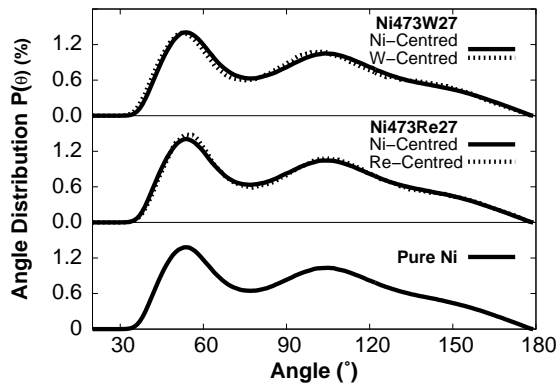
Figure 4: Angle distribution function P(\theta) at 1830 K for pure Ni, Ni_{473}Re_{27} and Ni_{473}W_{27} . For perfect icosahedral or bcc like structures the two main peaks are expected to be around 120 and 60 degrees, in our samples distortions due to the liquid nature shift the peaks to lower values. The angle distribution for all three cases of the Ni centered data fall on essentially the same line, and there is a slight shift to lower angles for the W centered distribution relative to the rest of the data.
